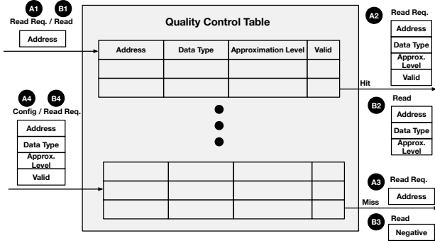
Figure 7: Hardware design of the quality control table: A1, A2, A3, and A4 represent packets encountered by the table at a core/L1 cache node. B1, B2, B3, and B4 represent packets encountered by the table at a memory/shared cache node.
