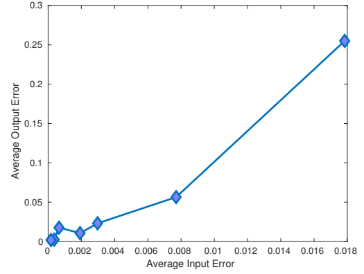
Figure 2: Relative errors on input data versus output data for the Black-Scholes benchmark: There is a clear linear relationship between the relative error on the input data and the relative error on the output data.
