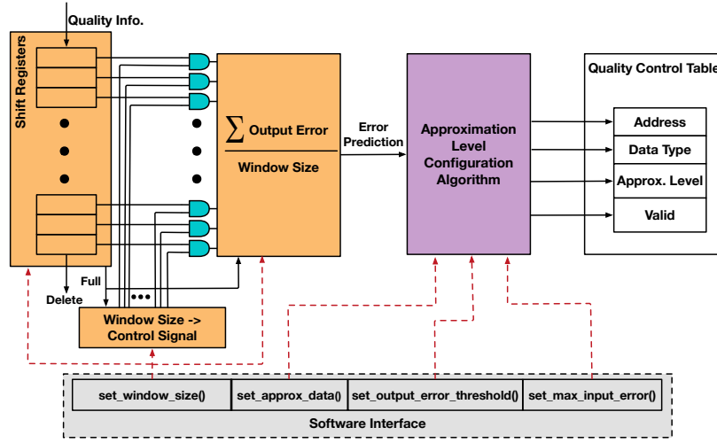
Figure 6: Hardware design of the approximation level configurator: Error prediction is accomplished by the orange part. Approximation level configuration is accomplished by the purple part.
