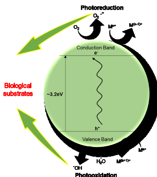
Figure 2. The semiconducting and photocatalytic properties of \text{TiO}_2 NPs.
