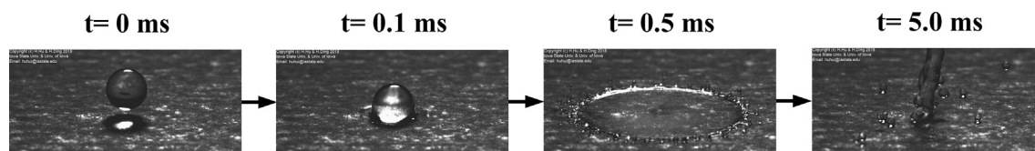
Fig. 4. Dynamic impinging test for nHSN treated superhydrophobic AA 6061 surface.
