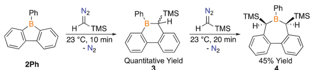
Scheme 1 Reaction of trimethylsilyldiazomethane with 2Ph .
