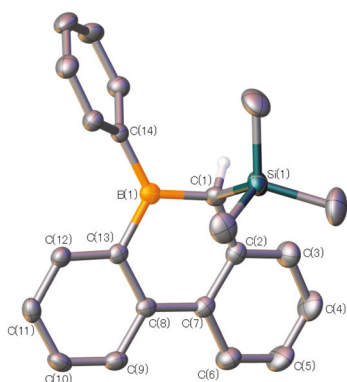
Fig. 3 Solid-state structure of 3 . Hydrogen atoms are omitted for clarity (except at the chiral center), and ellipsoids are drawn at the 50% probability level. Selected bond lengths (Å) and angles ( ^\circ ): B(1)–C(1) 1.541(3), C(1)–Si(1) 1.948(2), C(1)–C(2) 1.500(3), C(2)–C(7) 1.406(3), C(7)–C(8) 1.484(3), C(8)–C(13) 1.422(3), C(13)–B(1) 1.551(3), B(1)–C(14) 1.570(3), C(13)–B(1)–C(14) 122.26(18), C(13)–B(1)–C(1) 116.48(16), C(14)–B(1)–C(1) 121.17(16).
