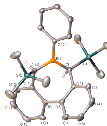
Fig. 4 Solid-state structure of 4 . Hydrogen atoms are omitted for clarity (except at chiral centers), and ellipsoids are drawn at the 50% probability level. Selected bond lengths (Å) and angles ( ^\circ ): B(1)–C(1) 1.587(3), C(1)–C(2) 1.523(2), C(2)–C(7) 1.409(3), C(7)–C(8) 1.486(3), C(13)–C(14) 1.509(2), C(14)–Si(2) 1.9302(17), C(14)–B(1) 1.567(3), B(1)–C(15) 1.568(3), C(14)–B(1)–C(15) 119.08(15), C(14)–B(1)–C(1) 117.36(15), C(15)–B(1)–C(1) 123.54(15).
