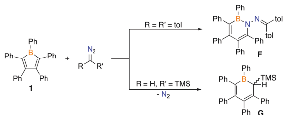
Fig. 2 Reactions of pentaphenylborole ( 1 ) with diazo reagents (tol = para -tolyl).
