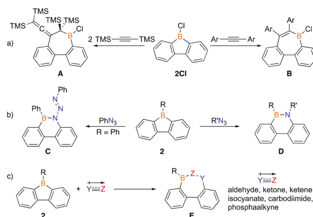
Fig. 1 Reported intermolecular insertion reactions of alkynes (a), azides (b), and unsaturated 1,2-dipolar molecules (c) with 9-borafluorenes. TMS = trimethylsilyl.
