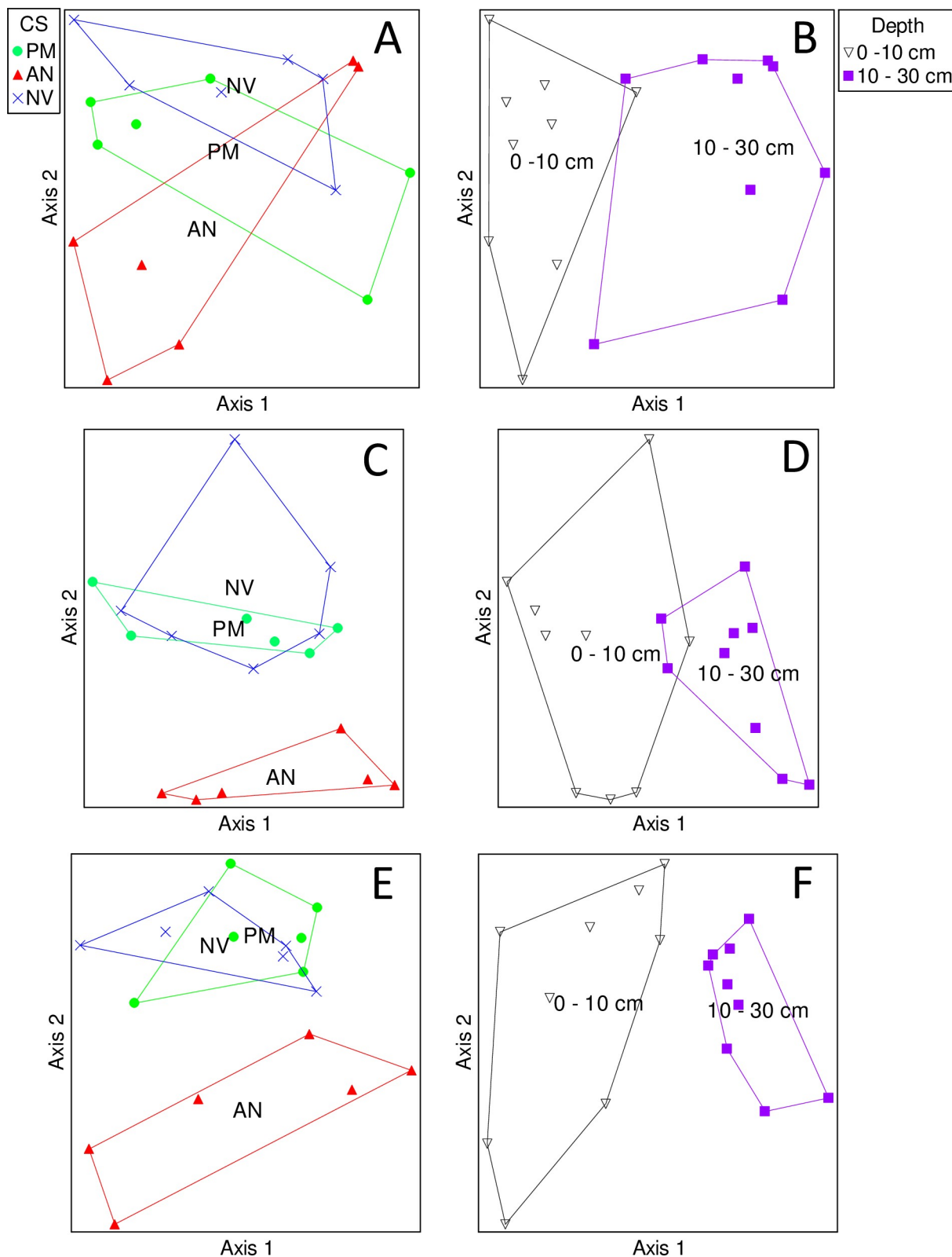
Fig 2. Nonmetric multidimensional scaling ordination of Pathotroph (A,B), Saprotroph (C,D), and Symbiotroph (E,F) OTUs sampled from plots of three cropping systems (CS: perennial monoculture (PM), annual agriculture (AN), native vegetation (NV)) and two soil depths (0–10 and 10–30 cm). The cropping system or depth label is at the centroid of each community.
