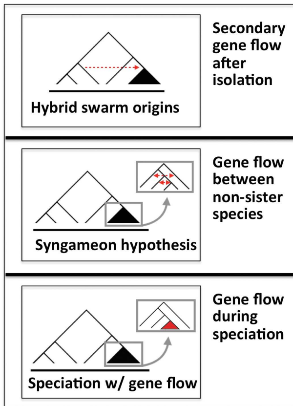
Figure 5. Gene flow, traditionally considered to hinder divergence between incipient species, can serve to infuse variability that may foster adaptive radiation. This can take place through (a) hybrid origins of entire radiating clades (“hybrid swarm origins”) wherein admixture between one or more divergent lineages happens prior to the onset of radiation, (b) via hybridization between nonsister species within adaptive radiations that facilitates further speciation (“syngameon hypothesis”) (Seehausen 2004), and (c) speciation with gene flow between sister species. It is important to distinguish between how admixture is achieved in order to assess its effects on the process of adaptive radiation (Brock and Wagner 2018). Both syngameon and hybrid swarm origins hypotheses have now been well documented in cichlid fish (Meier et al. 2017), and the importance of gene flow and the syngameon have been well demonstrated in Heliconius butterflies (Mallet 2005; Merrill et al. 2015), as well as many plants (Barrier et al. 1999; Friar et al. 2008), and are also found in many other lineages (Feder et al. 2003; Lamichhaney et al. 2018). Indeed, the processes may be common to many adaptive radiations. Moreover, there may be a “sweet spot” in which divergent lineages can admix or hybridize and give rise to variability that is key to adaptive radiation.
