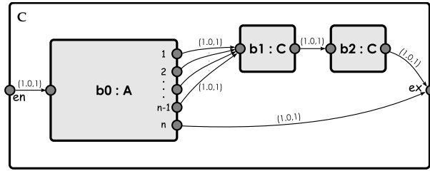
Fig. 3. Multi-exit reward RMDP: undecidability.
