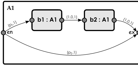
Fig. 2. Standard 1-RMC gadget used in proof of Theorem 19.
