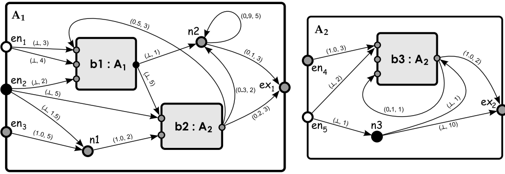
Fig. 1. A 1-RSSG example consisting of two components, A_1 and A_2 . Black vertices belong to player 1, white to player 2, grey vertices to “nature” (i.e., they are random). Each box (labelled, e.g., b1:A_1 ) has a name ( b1 ) and is mapped to a component ( A_1 ). Each edge has a label whose first component is \perp for controlled vertices or a probability value for random ones, and the second component is the reward assigned to this edge.
