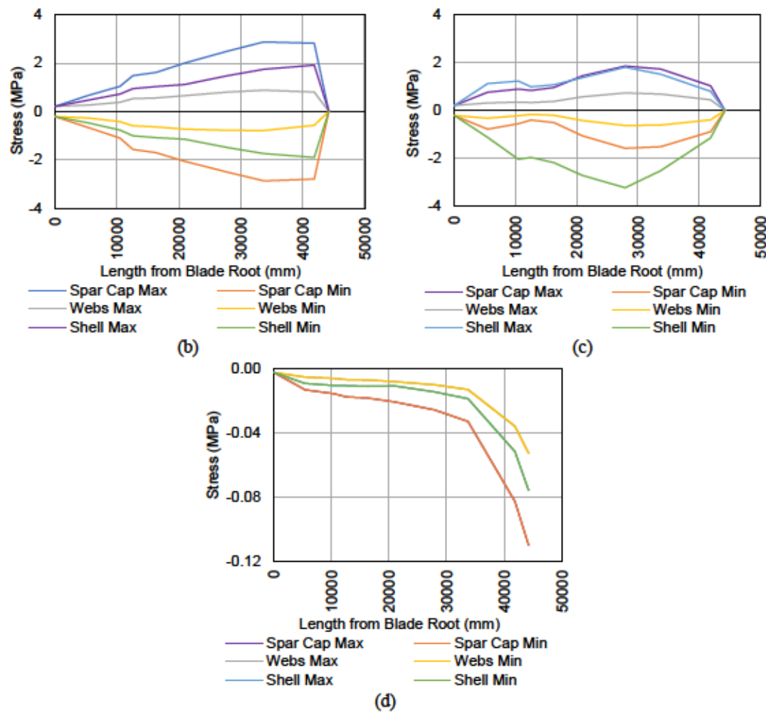
Figure 8. (a) Bending moment and axial force diagrams due to unit loads in the edgewise, flapwise, and axial directions, (b) Bending stresses due to flapwise bending, (c) bending stresses due to edgewise bending, and (d) axial compressive stresses.
