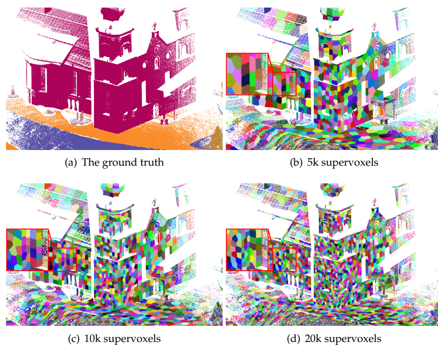
Figure 9. over-segmentation results with different numbers of supervoxels. (a) The ground truth; (b) 5000 supervoxels; BR = 0.4309 , UE = 0.1644 , GCE = 0.0174 ; (c) 10,000 supervoxels; BR = 0.5394 , UE = 0.1128 , GCE = 0.0122 ; and (d) 20,000 supervoxels; BR = 0.6217 , UE = 0.0784 , GCE = 0.0102 .
