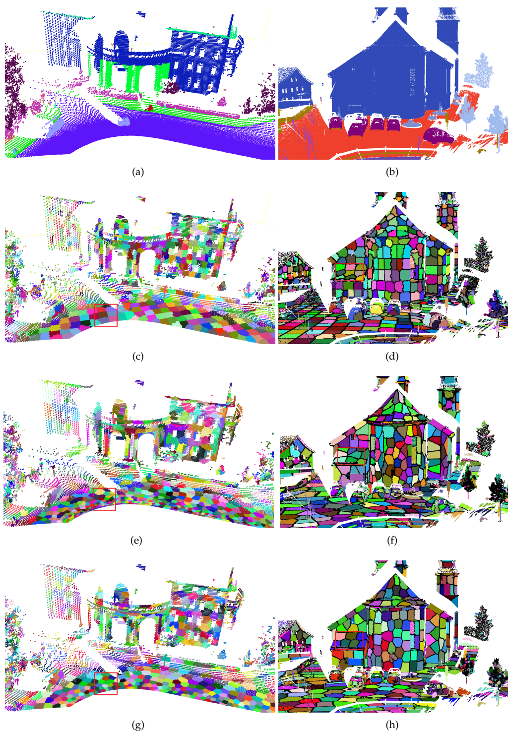
Figure 14. Visual comparisons using the point clouds from the Oakland (left) and Semantic3D (right) datasets. (a,b) Ground truth; (c,d) the VCCS results; (e,f) the BPSS results; and (g,h): our merge-swap results. Unlabelled points are not shown in the ground truth.
