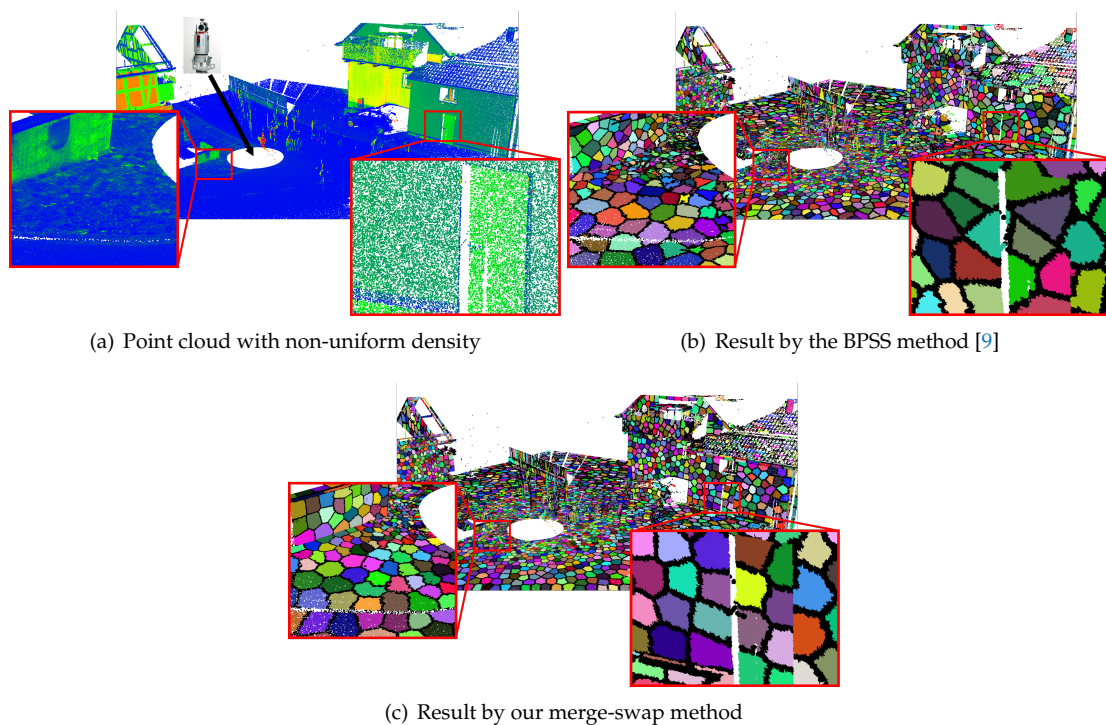
Figure 10. Comparison on a point cloud with non-uniform density. Our merge-swap method generates supervoxels with varying resolution and more regular shapes than the BPSS method.
