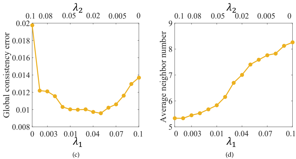
Figure 3. Effects of different combinations of weighting parameters \lambda_1 and \lambda_2 . We set (\lambda_1, \lambda_2) = (0.01, 0.05) by default in experiments. (a) Boundary recall; (b) under segmentation error; (c) global consistency error; and (d) average neighbor number.
