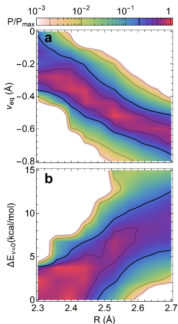
FIG. 6. Conditional probabilities (a) P_{cp}(R, v_{eq}) and (b) P_{cp}(R, \Delta E_{v=0}) from electronic structure calculations of 3665 SC-SC SHBs. In each graph, the probabilities are normalized by their maximum value.
