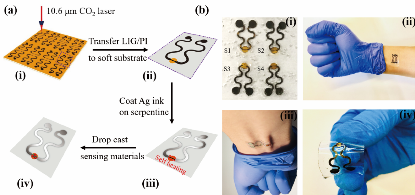
Figure 1. Schematic illustration of the fabrication process and demonstration of the wearable gas sensing platform. (a) Schematic illustration of the steps to prepare the stretchable LIG gas sensing platform: (i) porous LIG pattern on a PI film created by a laser scribing process, (ii) LIG/PI pattern transferred onto a soft elastomeric substrate, (iii) serpentine regions coated with conductive metal such as the Ag ink, (iv) gas-sensitive nanomaterials drop cast at the sensing region. (b) Optical images of the LIG gas sensing platform and its demonstration to follow various deformations applied to it. Various sensitive nanomaterials dispersed at the LIG sensing region could be designed with high selectivity to detect a specific component or with different selectivity to various components in the gaseous mixture upon various self-heating conditions. Collectively, the sensing response from the sensor array enables combinatorial sensing of multiple gas components in the mixture. Images of (i) a representative sensing platform with four sensing units arranged in an array of two by two on a soft substrate, (ii) sensing platform that followed the skin deformation from holding the fist, and deformations of a single sensing unit (iii) on the human wrist and (iv) in bending.
