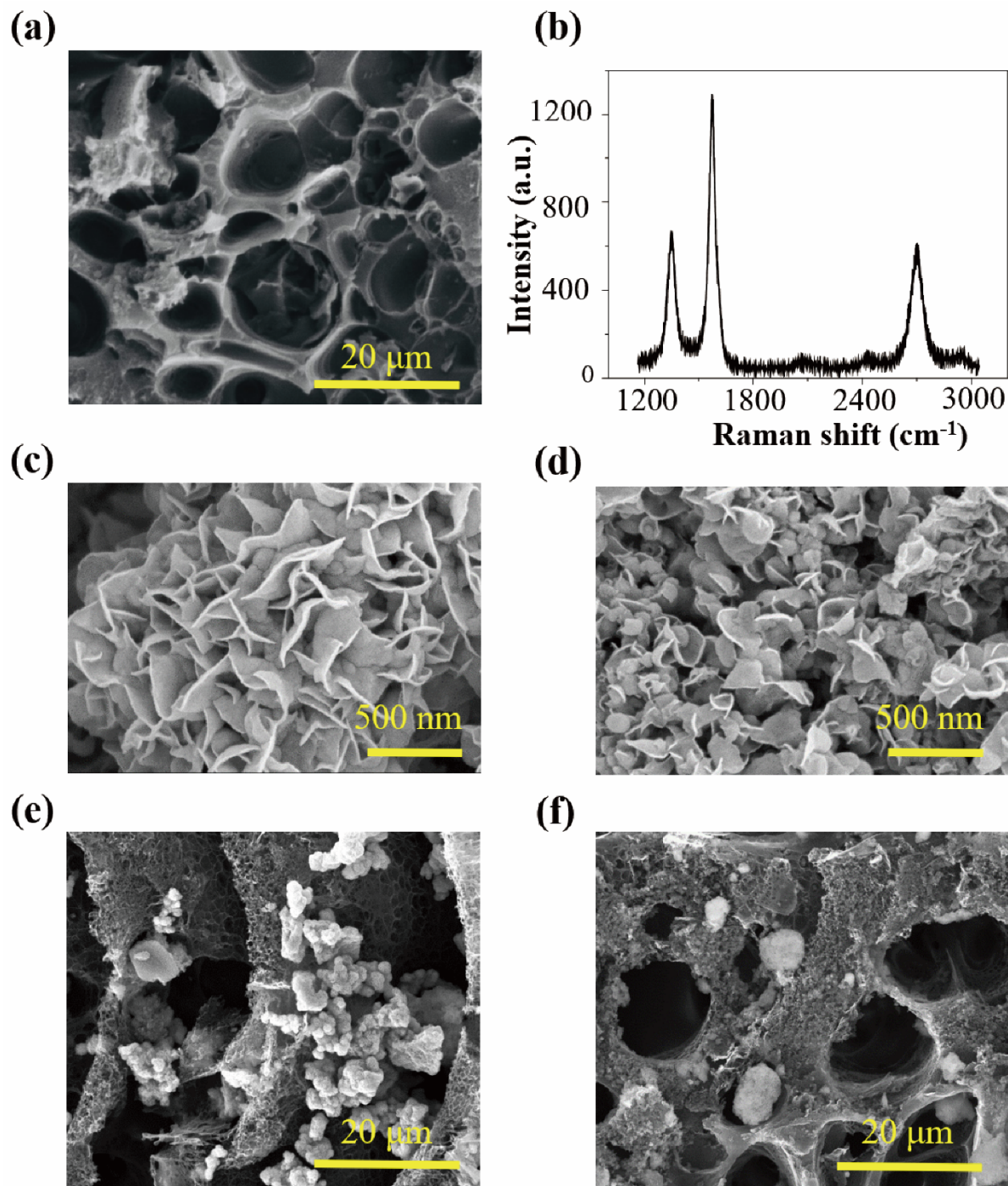
Figure 2. Characterization of the LIG gas sensing platform. (a) SEM image and (b) Raman spectrum of porous LIG electrode. SEM images of rGO/MoS 2 nanoflowers synthesized (c) without ("large petal") and (d) with ("small petal") the as-bought NaCl salt crystals. SEM images of rGO/MoS 2 nanoflowers with (e) "large petal" and (f) "small petal" structure dispersed on the porous LIG electrodes.
