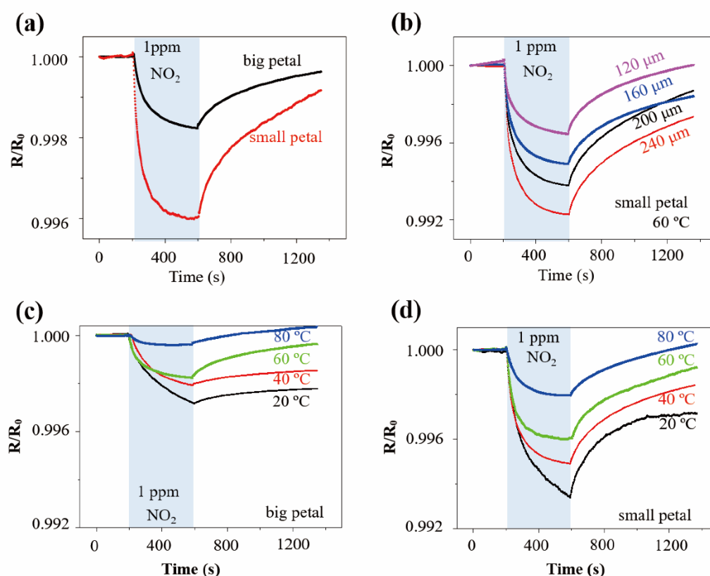
Figure 4. Effects of the width and operating temperature from self-heating on the gas sensing performance. (a) the typical response curves of rGO/MoS 2 nanoflowers with the small petal and big petal structure on the LIG sensing platform at 60 °C to NO 2 of 1 ppm. (b) Time-dependent response curves of rGO/MoS 2 nanoflowers with the small petal on the LIG with various widths at 60 °C. (c) Sensor response of rGO/MoS 2 nanoflowers with the big petal to 1 ppm NO 2 at various temperatures from self-heating. (d) Sensor response of rGO/MoS 2 nanoflowers with the small petal to 1 ppm NO 2 at various temperatures from self-heating.
