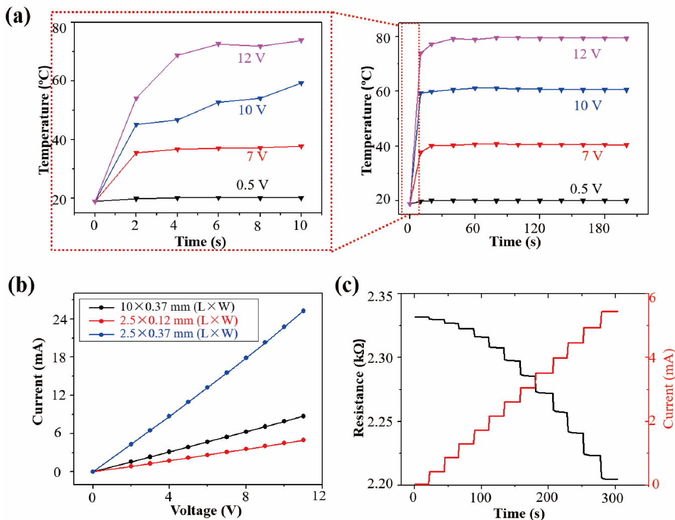
Figure 3. Characterization of the LIG electrode with self-heating capabilities. (a) The time-dependent temperature profile of the LIG electrode when different input voltages were applied during the resistance measurement of the chemiresistor. The inset shows the zoom-in of the measurement in the first 10 s. (b) Current-voltage (I-V) curves of three LIG electrodes with different sizes. (c) The change in resistance of and current in the LIG electrode with a length of 2.5 mm and width of 120 \mu m as a function of the time.
