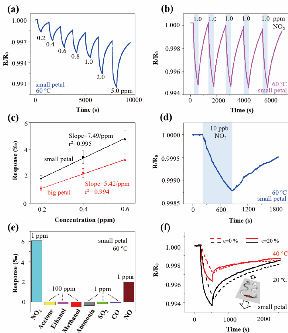
Figure 5. The dynamic response, limit of detection, selectivity, and mechanical robustness of the gas sensor. (a) Dynamic response test of the gas sensor with the small petal structure in the presence of NO 2 from 0.2 ppm to 5 ppm at 60 °C from self-heating (applied voltage of 10 V). (b) Demonstration of repeatability to NO 2 of 1 ppm for five consecutive cycles. (c) A linear fit to the calibration curves obtained from the sensor response to NO 2 of 200 ppb, 400 ppb, and 600 ppb at 60 °C from self-heating. (d) Experimental demonstration of the ultralow limit of detection to NO 2 of 10 ppb at 60 °C, where a high SNR of 62 was still measured. (e) The selectivity of the stretchable rGO/MoS 2 -LIG gas sensor to NO 2 over a wide range of other interfering gaseous molecules at 60 °C before stretching. (f) Response of the stretchable gas sensor in (e) to NO 2 of 1 ppm before and after a uniaxial tensile strain of 20 % was applied at room temperature and 40 °C, respectively.
