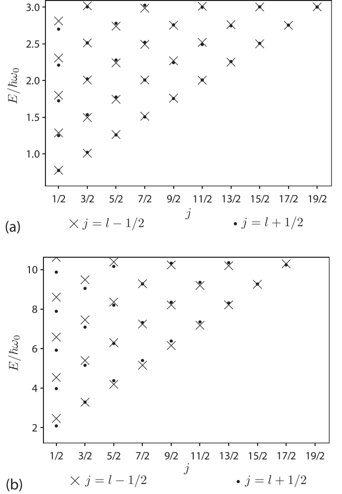
FIG. 2. Dependence of eigenenergies E_{n_r,j,l} on j for l = j \mp 1/2 and up to five lowest radial quantum numbers n_r . The harmonic trapping potential (43) is added. Panel (a) corresponds to a softer trap with \eta = 0.5 ; panel (b) corresponds to a tighter trap with \eta = 2 . The spectrum is calculated for the sinusoidal (26) driving for which \langle \cos(2r\mathcal{F}/r_0) \rangle = J_0(2r/r_0) .
