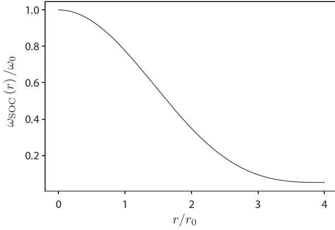
FIG. 1. Radial dependence of the SOC energy \omega_{\text{SOC}}(r) given by Eq. (35) for the sinusoidal driving (26) for which \langle \cos(2r\mathcal{F}/r_0) \rangle = J_0(2r/r_0) . The distance is measured in the units of r_0 and the frequency is measured in the units of the SOC frequency \omega_0 = \omega_{\text{SOC}}(0) given by Eq. (44).
