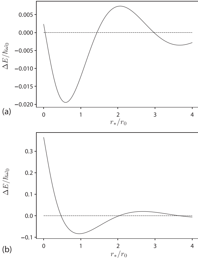
FIG. 3. Energy difference \Delta E = E_{j=\frac{1}{2}, l=1} - E_{j=\frac{1}{2}, l=0} vs the radius r_* of the additional hard core potential for an atom in a harmonic trapping potential (43) with \eta = 0.5 [panel (a)] and \eta = 2 [panel (b)]. The calculations are done for the sinusoidal driving (26) for which \langle \cos(2r\mathcal{F}/r_0) \rangle = \mathcal{J}_0(2r/r_0) .
