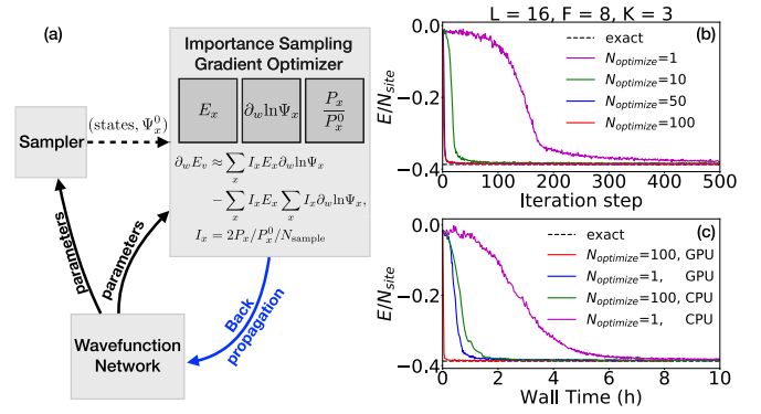
FIG. 3. (a) The flowchart of the ISGO algorithm within the VMC method. A network is used to represent the ground-state wave function. In every iteration step, the sampler generates N_{\text{sample}} samples following distribution P_x^0 \propto \Psi_x^{*0} \Psi_x^0 . Then the importance sampling optimizer updates the network parameters through back propagation in a loop for N_{\text{optimize}} times. N_{\text{optimize}} = 1 corresponds to the conventional gradient optimization method. The whole process is iterated until convergence. The sampler and the optimizer share the same wave function. We compare the training curves for a N_{\text{site}} = 60 SU(2) spin chain using a (L, F, K) = (16, 8, 3) CNN with one-hot encoding. (b) Variational energy vs iteration steps. (c) Variational energy vs wall time on GPU/CPU. The initial learning rate for Adam is 10^{-4} .
