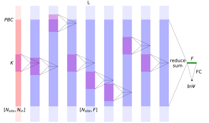
FIG. 1. The architecture of a convolutional DNN with L = 8 hidden layers. The input state is encoded into a 2D tensor of shape [N_{\text{site}}, N_{\text{in}}] , and fed into the input layer (represented by the leftmost pink rectangle). For value encoding N_{\text{in}} = 1 and for one-hot encoding N_{\text{in}} = N . The blue rectangles stand for the activation (feature maps) of the hidden layers. Convolution filters (the small pink rectangles) transform one hidden layer to the next one. The last hidden layer (on the right) is reduce summed and followed by a fully connected layer to give the \ln \Psi output.
