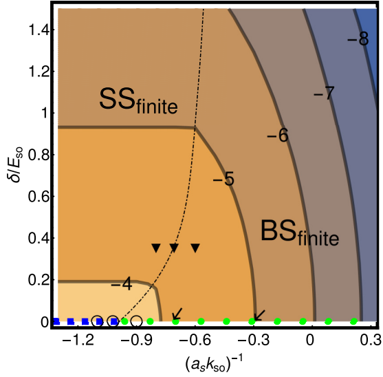
FIG. 9. “Phase diagram” for the total ground state as functions of (a_s k_{so})^{-1} and \delta/E_{so} for \Omega = 2E_{so} . The contours show the total ground-state energy E_3^{(0)}(q_{3,z})/E_{so} . The black dot-dashed line, the green circles, and the blue squares separate the two phases SS_{finite} and BS_{finite} from each other. The open circles and triangles mark the parameter combinations corresponding to Figs. 7(a) and 7(b). The arrows mark the scattering lengths corresponding to Figs. 8(a) and 8(b).
