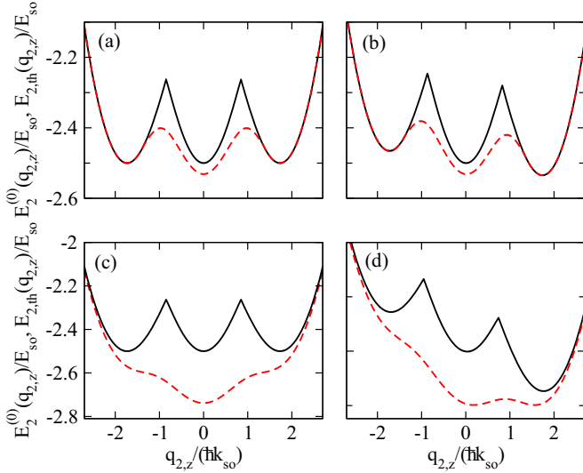
FIG. 3. The ground-state energy E_2^{(0)}(q_{2,z}) of \hat{H}_N(q_{2,z}) (red dashed lines) and the threshold energy E_{2,th}(q_{2,z}) (black solid lines) for \Omega = 2E_{so} and various (a_s k_{so})^{-1} and \delta/E_{so} combinations. Panels (a) and (b) correspond to (a_s k_{so})^{-1} = -0.321 . Panels (c) and (d) correspond to (a_s k_{so})^{-1} = 0.0113 . Panels (a) and (c) correspond to \delta = 0 . Panel (b) and (d) correspond to \delta = 0.04E_{so} and \delta = 0.21E_{so} , respectively.
