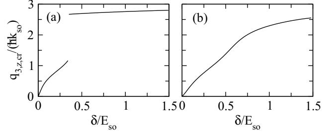
FIG. 8. The critical center-of-mass momentum q_{3,z,\text{cr}} of the three-boson ground state as a function of \delta/E_{so} for \Omega = 2E_{so} and (a) (a_s k_{so})^{-1} = -0.72 and (b) (a_s k_{so})^{-1} = -0.3 .
