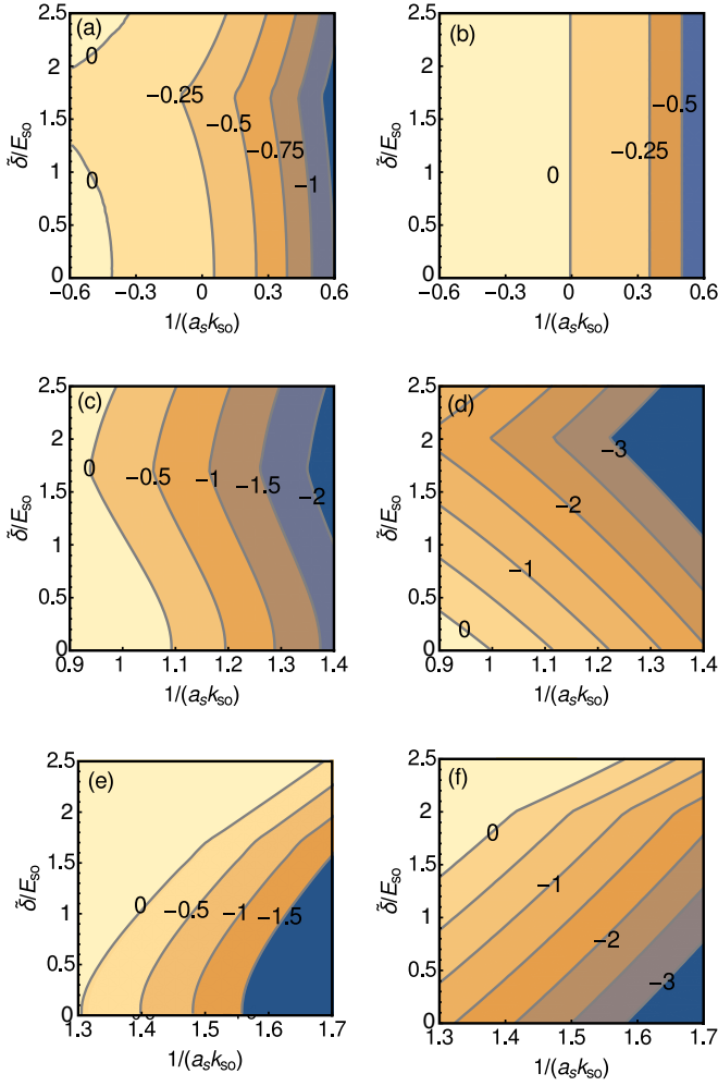
FIG. 1. The contours show the negative of the two-boson binding energy, in units of E_{so} , as functions of (a_s k_{so})^{-1} and \tilde{\delta}/E_{so} for \Omega = 2E_{so} [panels (a), (c), and (e)] and infinitesimally small \Omega [panels (b), (d), and (f)]. The panels in the first row, second row, and third row show the negative of the binding energy of the energetically lowest-lying two-boson state ( n = 0 ), of the first-excited two-boson state ( n = 1 ), and of the second-excited two-boson state ( n = 2 ). Note the different ranges of the x axis in panels (a)–(f).
