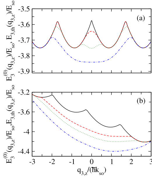
FIG. 7. The ground-state energy E_3^{(0)}(q_{3,z}) of \hat{H}_3(q_{3,z}) and the threshold energy E_{3,\text{th}}(q_{3,z}) for \Omega = 2E_{so} and various (a_s k_{so})^{-1} and \delta/E_{so} combinations. The black solid lines correspond to E_{3,\text{th}}(q_{2,z}) . The red dashed, green dotted, and blue dot-dashed lines in panel (a) show E_3^{(0)}(q_{3,z}) for \delta = 0 and (a_s k_{so})^{-1} = -1.1, -1.02 , and -0.9 , respectively. The red dashed, green dotted, and blue dot-dashed lines in panel (b) show E_3^{(0)}(q_{3,z}) for \delta = 0.35E_{so} and (a_s k_{so})^{-1} = -0.8, -0.72 , and -0.6 , respectively.
