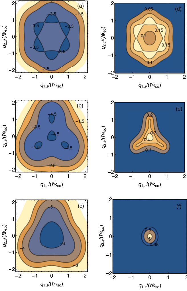
FIG. 6. Correlations between the lowest noninteracting relative dispersion curve and the relative momentum distribution for the ground state for \Omega = 2E_{so} and (a_s k_{so})^{-1} = -0.96 . Panels (a)–(c) show the lowest noninteracting relative dispersion curves for \tilde{\delta} = 0 , 2.27E_{so} , and 3.5E_{so} , respectively. Panels (d)–(f) show the relative momentum distributions for the ground state for \tilde{\delta} = 0 , 2.27E_{so} , and 3.5E_{so} , respectively. Note that the contours in panels (a)–(e) are equally spaced while those in panel (f) are not.
