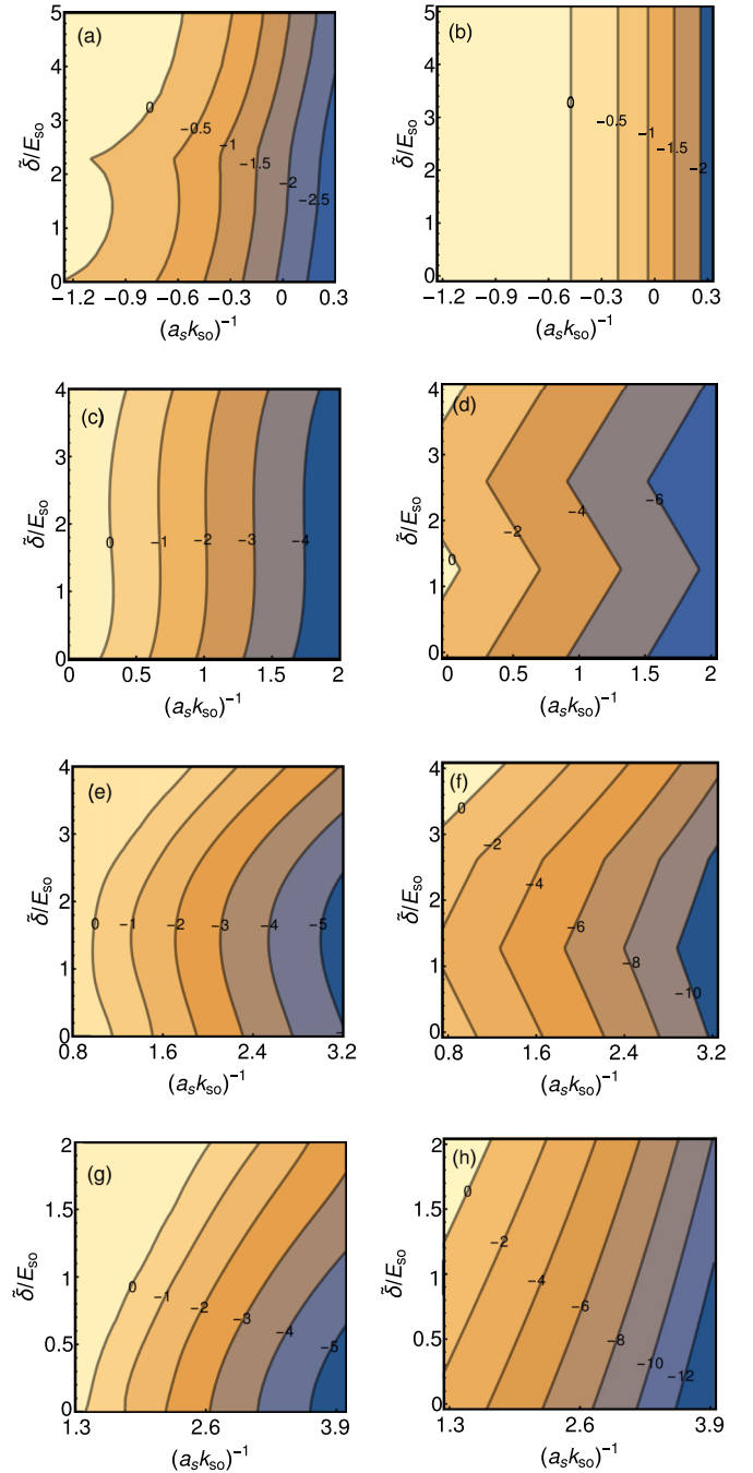
FIG. 5. The contours show the negative of the three-boson binding energy, in units of E_{\text{so}} , as functions of (a_s k_{\text{so}})^{-1} and \tilde{\delta}/E_{\text{so}} for k_{\text{so}}/\kappa_* = 1.32 and \Omega = 2E_{\text{so}} [panels (a), (c), (e), and (g)] and infinitesimally small \Omega [panels (b), (d), (f), and (h)]. Panels in the first, second, third, and fourth row show the negative of the binding energy for the three-boson states with n = 0, 1, 2 , and 3 , respectively. Note the different ranges of the x axis in panels (a)–(h). The four states n = 0-3 correspond to the lowest Efimov manifold. Applying the generalized radial scaling law [41], these energy plots also describe higher-lying Efimov manifolds.
