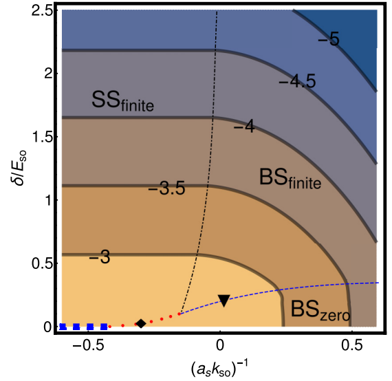
FIG. 4. “Phase diagram” for the total ground state as functions of (a_s k_{so})^{-1} and \delta/E_{so} for \Omega = 2E_{so} . The contours show the total ground-state energy E_2^{(0)}(q_{2,z})/E_{so} . The black dot-dashed line, blue dashed line, red dotted line, and the blue squares separate the three phases SS_{finite} , BS_{finite} , and BS_{zero} from each other (see text for details). The diamond and triangle mark the parameter combinations corresponding to Figs. 3(b) and 3(d), respectively.
