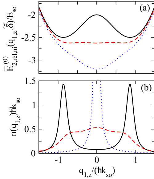
FIG. 2. Correlations between (a) the lowest noninteracting relative dispersion curve and (b) the relative momentum distribution for the ground state with \Omega = 2E_{so} and (a_s k_{so})^{-1} = -0.321 . For both panels, the black solid, red dashed, and blue dotted lines correspond to \tilde{\delta} = 0 , 1.7E_{so} , and 2.5E_{so} , respectively.
