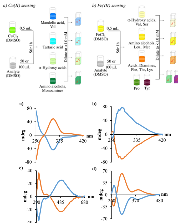
Fig. 2 General workflow of the CD sensing assay and examples of ICD effects obtained for 1 (a), 15 (b), 8 (c) and 17 (d) using Pd(NO 3 ) 2 , FeCl 2 , FeCl 3 and CuCl 2 , respectively. The sensing with Pd(II) was conducted at 1.8 mM in MeOH. All other spectra were collected at 0.5 mM in DMSO.
