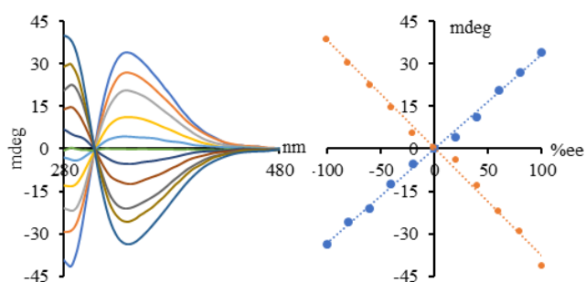
Fig. 3 ICD sensing of tartaric acid samples of varying enantiomeric composition with \text{FeCl}_3 and plot of the induced maxima at 288 (red) and 338 (blue) nm versus sample ee (0.5 mM, DMSO).
