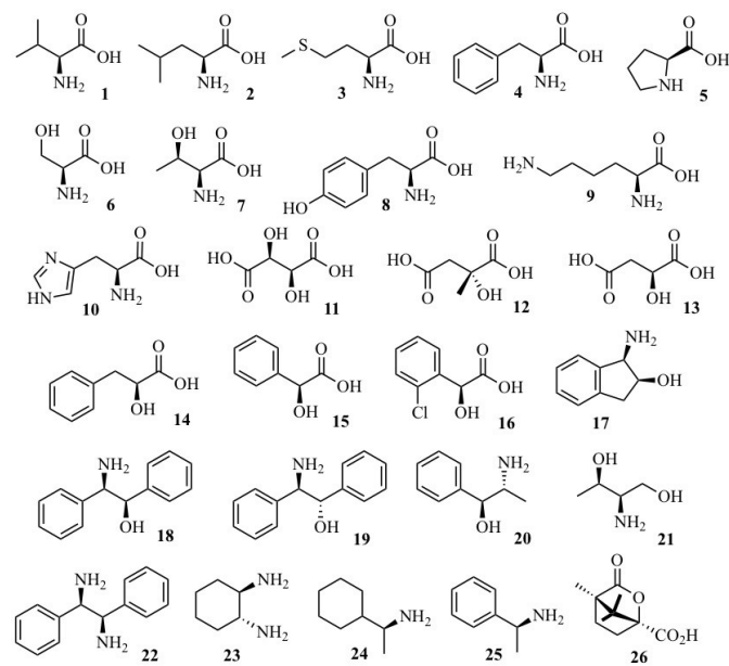
Fig. 1 Structures of chiral ligands tested. Only one enantiomer is shown.
