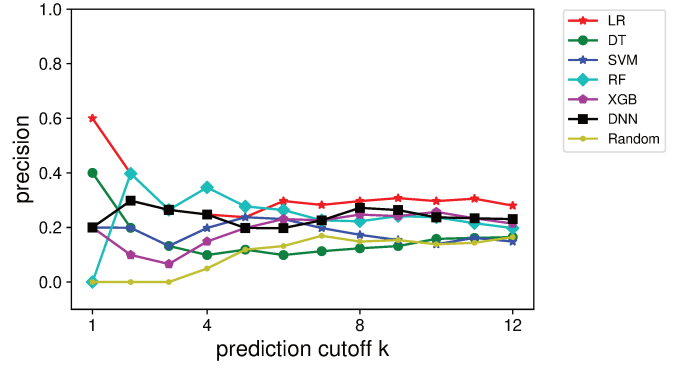
Figure 12: Average precision@k for post dataset.
