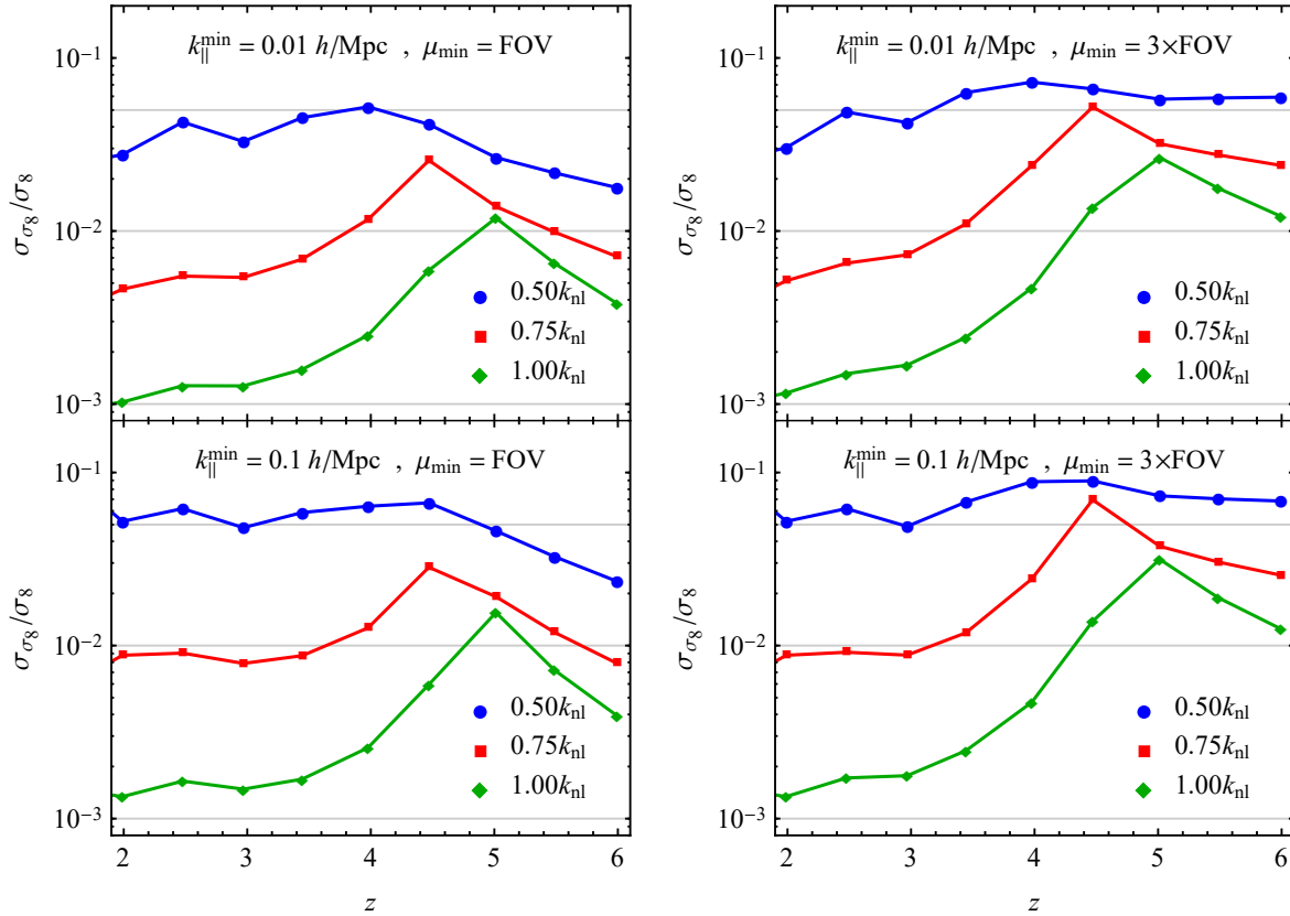
Figure 5: Forecast fractional error on the power spectrum normalization, \sigma_8 , from a future 21-cm experiment. The left panels show an optimistic scenario with good foreground cleaning of the wedge, and two choices of k_{\parallel}^{\min} , while the right panel shows a pessimistic scenario. Blue lines show constraints from k_{\max} = 0.50 k_{\text{nl}} while red lines show k_{\max} = 0.75 k_{\text{nl}} and green those for k_{\max} = 1.00 k_{\text{nl}} . These span the range of likely possibilities.
