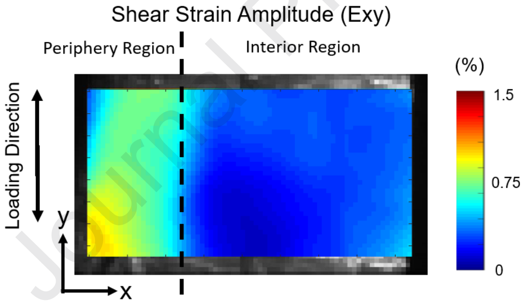
Figure 4: Local shear strains caused by shear loading in a 5 week construct
