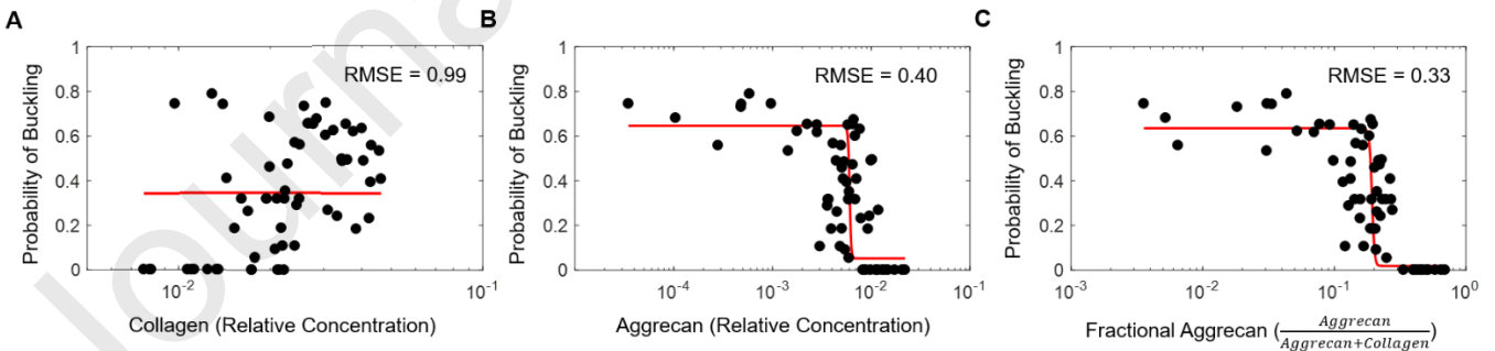
Fig 7: The relationship between local construct buckling and biochemical content follows a sigmoidal function A) Collagen concentration does not affect buckling (RMSE = 0.99). B) The buckled fraction at a given depth stays constant until a threshold of aggrecan is reached at 0.0060, at which point buckling does not occur (RMSE = 0.40). C) The ratio of aggrecan to collagen content in engineered cartilage constructs reveals a threshold at 0.19 between buckled and non-buckled locations (RMSE = 0.33, N = 61)
