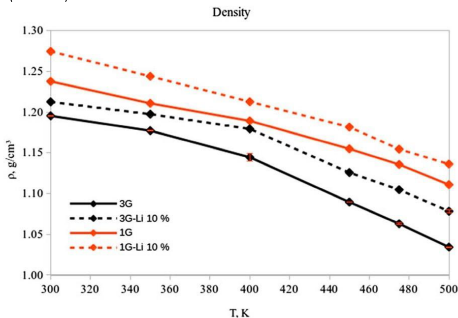
Figure 12. Calculated density at different temperatures for [sPyr + ][BF 4 − ] using one and three polarizable groups for 300–500 K. Reproduced from Torabifard, H.; Reed, L.; Berry, M.T.; Hein, J.E.; Menke, E.; Cisneros, G.A. Computational and Experimental Characterization of a Pyrrolidinium-Based Ionic Liquid for Electrolyte Applications. J. Chem. Phys. 2017 , 147 , 161731 [105].
