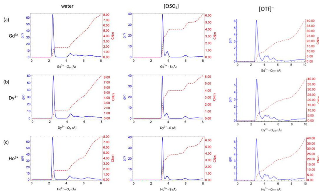
Figure 3. Radial distribution functions and integration curves of water (left) [EtSO 4 ] (center) and [OTf] (right) around the lanthanide cations. Reproduced from Tu, Y.-J.; Allen, M.J.; Cisneros, G.A. Simulations of Water Exchange Dynamics on Lanthanide Ions in 1-Ethyl-3-Methylimidazolium Ethyl Sulfate ([EMIm][EtSO 4 ]) and Water. Phys. Chem. Chem. Phys. 2016 , 18 , 30323–30333. With permission from the PCCP Owner Societies [103], and Tu, Y.-J.; Lin, Z.; Allen, M.J.; Cisneros, G.A. Molecular Dynamics Investigation of Solvent-Exchange Reactions on Lanthanide Ions in Water/1-Ethyl-3-Methylimidazolium Trifluoromethylsulfate ([EMIm][OTf]). J. Chem. Phys. 2018 , 148 , 024503. Copyright 2018 American Physical Society.
