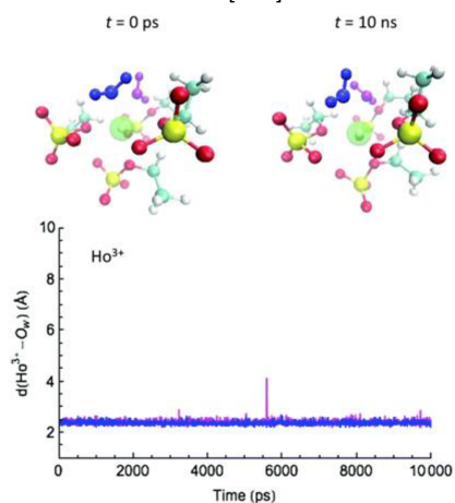
Figure 5. Selected snapshots for a water exchange event on Ho 3+ in water/[EMIm][EtSO 4 ] and corresponding cation—water distance along the MD trajectory. Similar behaviors were observed for Gd 3+ and Dy 3+ . Reproduced from Tu, Y.-J., Allen, M.J., Cisneros, G.A., (2016) “Simulations of Water Exchange Dynamics on Lanthanide Ions in 1-Ethyl-3-Methylimidazolium Ethyl Sulfate ([EMIm][EtSO 4 ]) and Water”, Phys. Chem. Chem. Phys. , 18 , 30323–30333. with permission from the PCCP Owner Societies [103].
