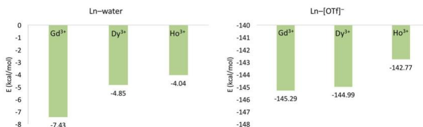
Figure 7. Average total interaction energies of lanthanide ions with a [OTf] − anion and a first shell (a) and second shell (b) water. Reproduced from Tu, Y.-J.; Lin, Z.; Allen, M.J.; Cisneros, G.A. Molecular Dynamics
