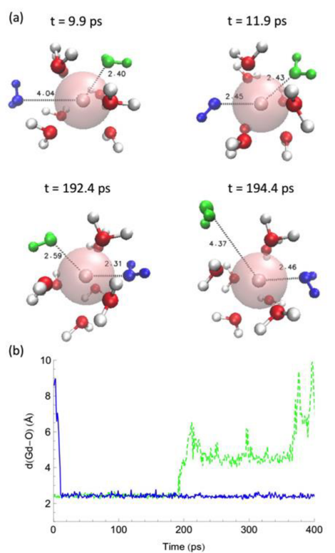
Figure 4. (a) Selected snapshots for a water exchange event on Gd 3+ in water and (b) corresponding cation—water distance along the MD trajectory. A similar behavior is observed for Dy 3+ and Ho 3+ in water.
