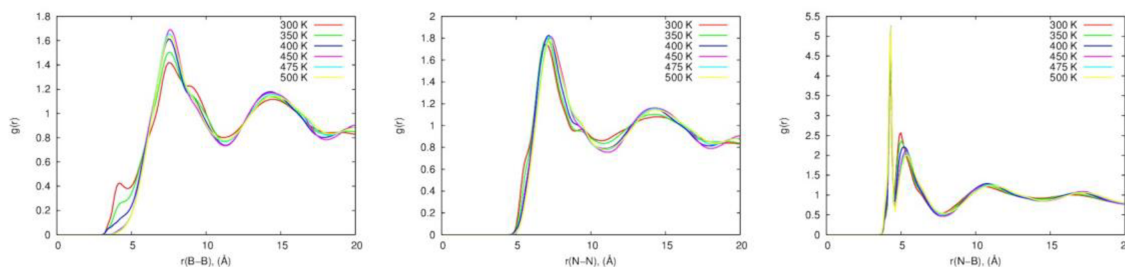
Figure 13. Radial distribution functions for [sPyr+][BF 4 − ] with three polarizable groups (3G) at different temperatures. Reproduced from Torabifard, H.; Reed, L.; Berry, M.T.; Hein, J.E.; Menke, E.; Cisneros, G.A. Computational and Experimental Characterization of a Pyrrolidinium-Based Ionic Liquid for Electrolyte Applications. J. Chem. Phys. 2017 , 147 , 161731, [105].
