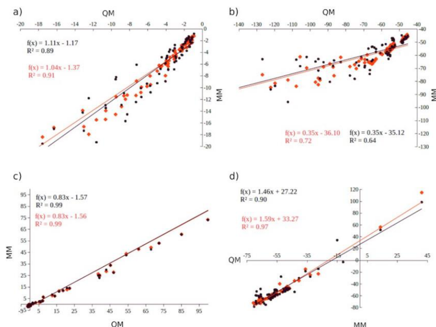
Figure 1. (a) polarization, (b) Coulomb, (c) Van der Waals and (d) Total inter-molecular interaction energies for 77 randomly oriented [sPyr+][BF 4 ] dimers computed with AMOEBA-IL (MM) compared with QM EDA (SAPT) with (black), or without (red) inter-molecular polarization. Reproduced from Torabifard, H.; Reed, L.; Berry, M.T.; Hein, J.E.; Menke, E.; Cisneros, G.A. Computational and Experimental Characterization of a Pyrrolidinium-Based Ionic Liquid for Electrolyte Applications. J. Chem. Phys. 2017 , 147 , 161731. [105].
