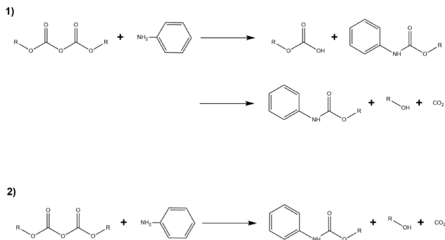
Figure 15. Reaction scheme for the N-tert -butoxycarbonylation of aniline. Panel (1) describes the step-wise mechanism and panel (2) describes the concerted mechanism mentioned above.
