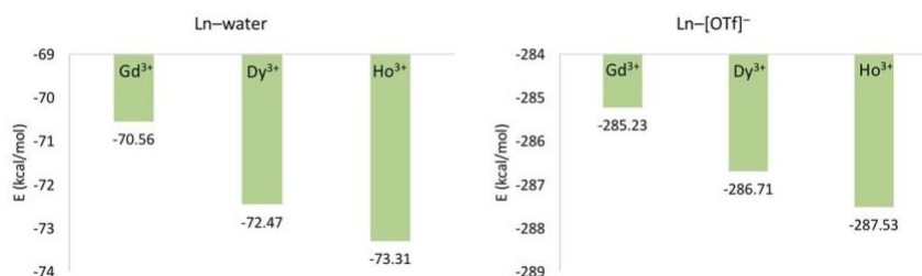
(b) The second solvation shell
