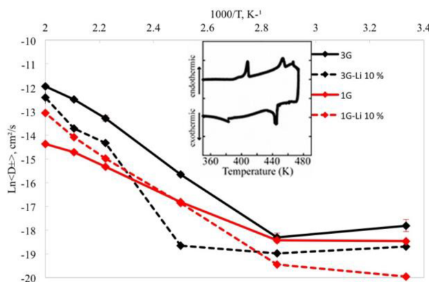
Figure 14. Calculated diffusion coefficients at different temperatures for [sPyr + ][BF 4 − ] using one (1G) and three (3G) polarizable groups with and without 10% Li + . Reproduced from Torabifard, H.; Reed, L.; Berry, M.T.; Hein, J.E.; Menke, E.; Cisneros, G.A. Computational and Experimental Characterization of a Pyrrolidinium-Based Ionic Liquid for Electrolyte Applications. J. Chem. Phys. 2017 , 147 , 161731 [105].
