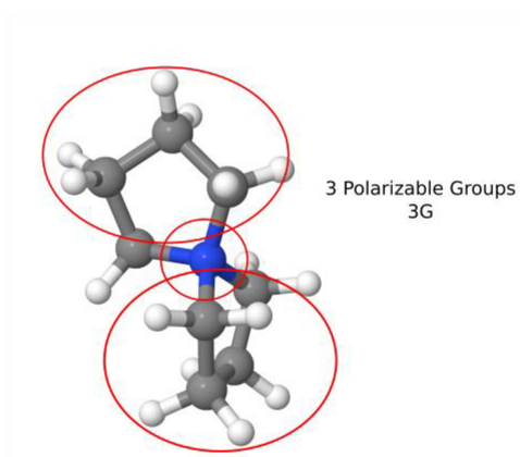
Figure 2. Spirocyclic pyrrolidinium [SPyr] molecular structure, red circles roughly denote the intra-molecular polarization groups for the 3G set, from Torabifard, H.; Reed, L.; Berry, M.T.; Hein, J.E.; Menke, E.; Cisneros, G.A. Computational and Experimental Characterization of a Pyrrolidinium-Based Ionic Liquid for Electrolyte Applications. J. Chem. Phys. 2017 , 147 , 161731. [105].
