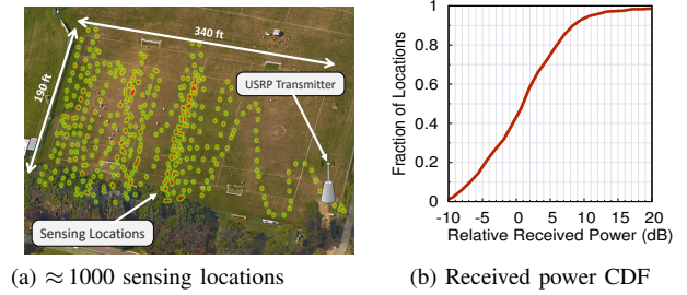
Figure 5: Spectrum sensor data collection
