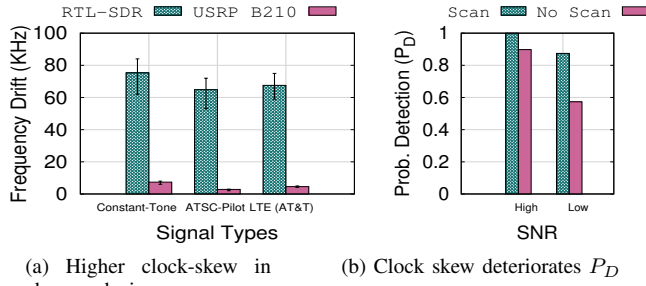
Figure 3: Unpredictable clock skew makes frequency offset calculation harder resulting in poorer signal detection performance.
