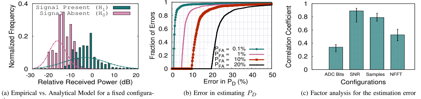
Figure 6: Analysis of estimation errors associated with analytical models and its dependency on the sensor's operating environment or configurations. Median estimation error in P_D can be as high as 25%. Higher errors are highly associated to low SNR operating environments.
