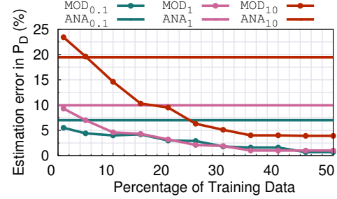
Figure 7: Performance of the data-driven models MOD_{P_{FA}} compared to the analytical models ANA_{P_{FA}} for different values of P_{FA} .
