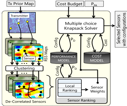
Figure 10: Schematic of the sensor selection technique
