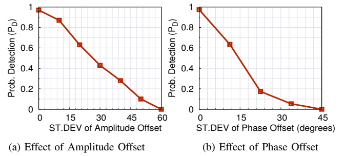
Figure 4: We demonstrate the effect of I/Q imbalance in deteriorating the performance of simple waveform based detector algorithm used in detecting an ATSC pilot tone.
