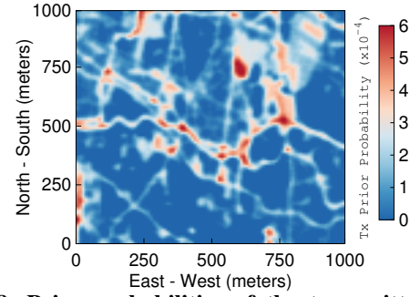
Figure 8: Prior probabilities of the transmitter across a 1000 m × 1000 m grid.
