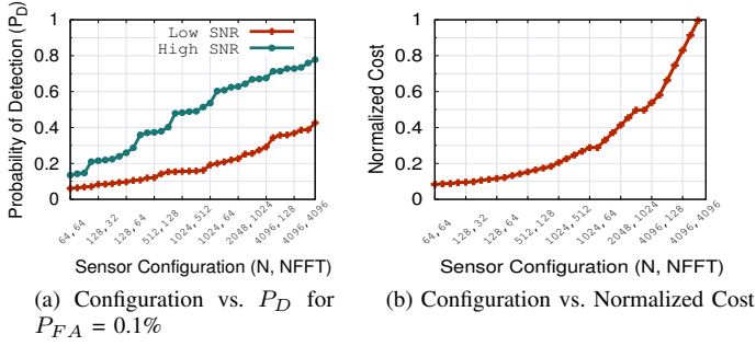
Figure 9: (a) P_D for different configurations of the sensor under low and high SNR. (b) Sensor cost model. N is number of samples, NFFT is no. of FFT bins.
