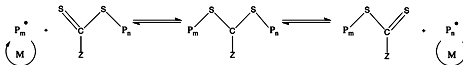
Scheme 3. Generalized RAFT Reaction Mechanism
