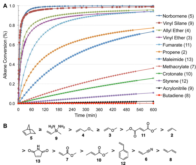
Figure 3. Effect of alkene group selection on thiol-ene reaction kinetics. (A) Theoretical computation of the kinetics of the thiol-ene reaction dependent on the reactivity of the chosen alkene group. Norbornene is a popular alkene candidate for thiol-ene reactions due to its superior reaction rate. Methacrylate, the common reactive group for chain-growth photopolymerization, has a starkly slow thiol-ene kinetics, with the alkene conversion well below 50% even after a 10 h reaction time. (B) Descending list of alkene group reactivity based on the theoretical kinetics model. Reprinted with permission from ref 67. Copyright 2012 American Chemical Society.
