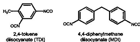
Figure 11. Common diisocyanates used in large-scale polyurethane productions.
