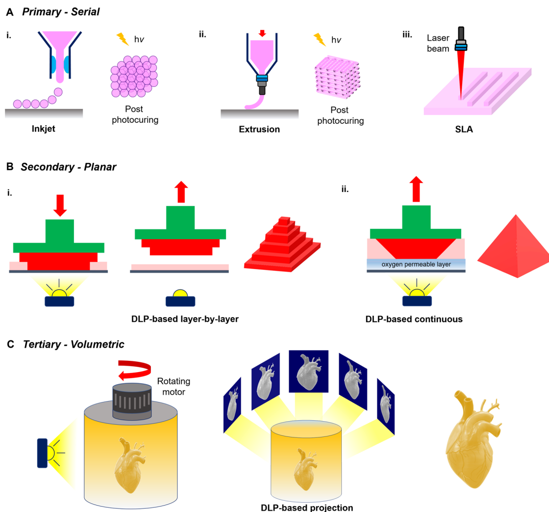
Figure 20. Classification of light-based 3D printing modalities. (A) Primary configuration involves serial deposition of biomaterials in dot-by-dot or line-by-line fashion. (B) Secondary configuration involves planar build via digital light processing (DLP)-based projection of patterns into a biomaterial vat. (C) Tertiary configuration involves volumetric build via DLP-based projection of patterns into a rotating biomaterial vat.
