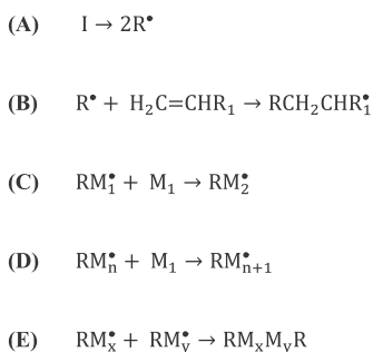
Scheme 1. General Initiation (A,B), Propagation (C,D), and Termination (E) Chemical Reactions for Free Radical Polymerization
