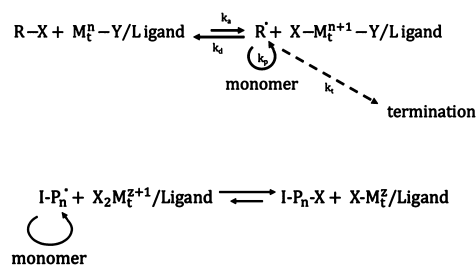
Scheme 2. (top) Generalized ATRP Reaction Mechanism; (bottom) Generalized Reverse-ATRP Reaction Mechanism
