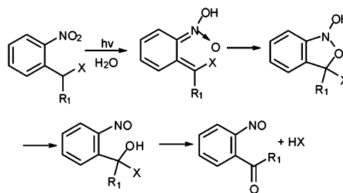
Figure 5. Photolysis mechanism of o -nitrobenzyl ( R_1 = H ) and nitrophenylethyl ( R_1 = \text{methyl} ).
