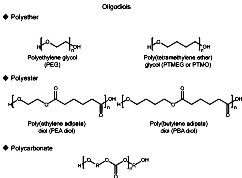
Figure 12. Common oligodiols used in polyurethane production, including polyether, polyester, and polycarbonate-based oligodiols. The nature of oligodiols used will determine the properties of polyurethane synthesized.
