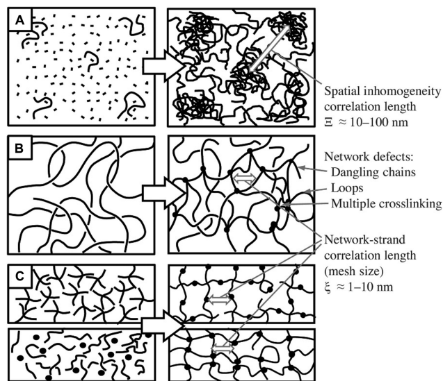
Figure 4. Depiction of hydrogel network formation depending on cross-linking mechanism and the resulting degree of inhomogeneity. (A) Free-radical chain growth polymerization of monomers and cross-linkers leading to spatial inhomogeneity within the network architecture. (B) Network formation via cross-linking of reactive functional side groups of the polymer chains in a semidilute solution, leading to local inhomogeneity. (C) Orthogonal step-growth polymerization resulting in a mostly ordered, homogeneous network. Reproduced with permission from ref 78. Copyright 2017 Elsevier.
