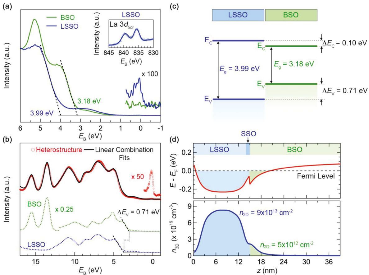
Figure 3. Band alignment at LSSO/SSO/BSO interface. (a) VB spectra of the reference BSO (green) (56 nm BSO/STO (001)) and LSSO (blue) (41 nm LSSO/8 nm SSO/GSO (110)) films. Electronic states near the Fermi states are magnified. Inset shows the La 3d_{5/2} core-level X-ray photoelectron spectra, (b) VB spectra of the SSO/BSO heterostructure (red) along with the fit (black) using linear combination of the reference VB spectra (dotted green and blue lines) to determine the VB offset. (c) Energy-level flat-band diagram showing the measured band offsets between LSSO and BSO, and (d) conduction band minima (red) referenced to the Fermi level (top panel) and 3D carrier density, n_{3D} (blue) as a function of depth for the SSO/BSO (bottom panel). The shaded regions indicate 2D density in LSSO and BSO layers after the charge transfer.
