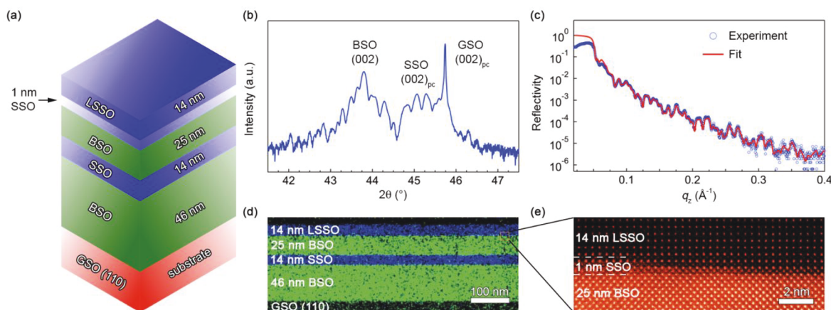
Figure 1. Structural characterization of \text{SrSnO}_3/\text{BaSnO}_3 heterostructure. (a) Schematic of the \text{SrSnO}_3/\text{BaSnO}_3 heterostructure grown on GSO (110), (b) wide-angle X-ray diffraction (WAXRD), (c) grazing incidence X-ray reflectivity of the heterostructure along with a fit using GenX software, (d) energy dispersive X-ray (EDX) elemental maps of Ba L_\alpha (green) and Sr L_\alpha (blue) in the heterostructure, (e) HAADF-STEM image of the top LSSO/SSO/BSO interface.
