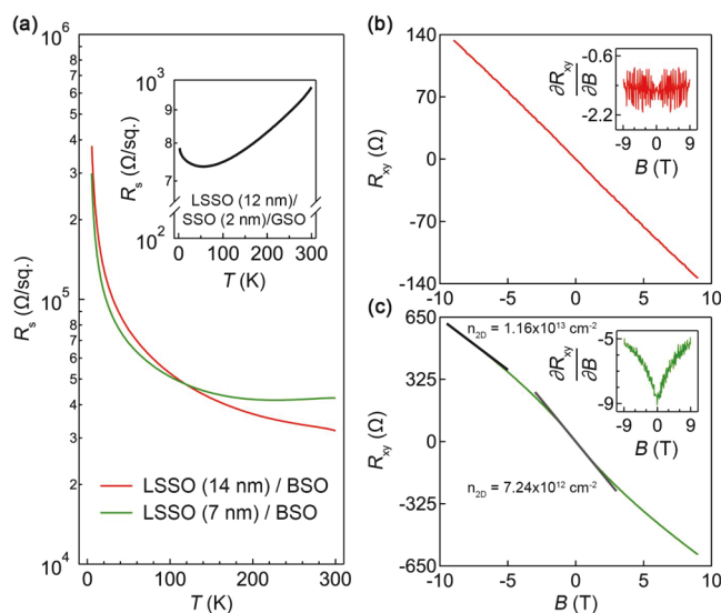
Figure 2. Electrical transport in \text{SrSnO}_3/\text{BaSnO}_3 heterostructures. (a) R_s versus T for the LSSO/BSO heterostructures with \sim 14 nm LSSO (red) and 7 nm LSSO (green). Inset shows the R_s versus T behavior for 12 nm LSSO/2 nm SSO/GSO (110) without BSO interface layer as a reference. (b,c) Transverse resistance ( R_{xy} ) as a function of B at 30 K for the two heterostructures. Insets show the corresponding first derivatives of R_{xy} with respect to B ( \partial R_{xy}/\partial B in \text{m}\Omega/\text{G} ) versus B .
