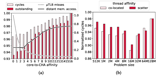
Figure 3: Effects of core-to-CHA and core-to-core affinities: 3a) execution cycles, outstanding weighted cycles, \mu TLB misses, and accesses to distant memory interfaces for different core-to-CHA affinities. Results are normalized to the maximum value for each series, except for accesses to distant memory interfaces, which are normalized to the total number of memory accesses. \mu TLB misses and distant accesses are referenced to the right axis; and 3b) execution cycles of the best-performing CHA-to-core affinity for two different core-to-core affinities: “scatter” (thread i is assigned to OS core i ), and “co-located” (adjacent threads are placed in adjacent physical cores). Results are normalized to the execution cycles of the non-optimized code with scatter thread placement. The left Y axes are truncated to better reflect the differences in values.
