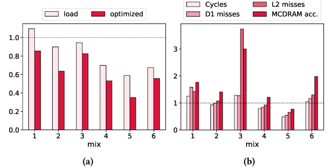
Figure 4: Results of optimized scheduling methodologies: 4a) Execution cycles of “load” and “optimized” schedules normalized to “fair” values; and 4b) Performance counters of “optimized” schedules aggregated over the sum of each mix and normalized to the values in “fair” schedules.
