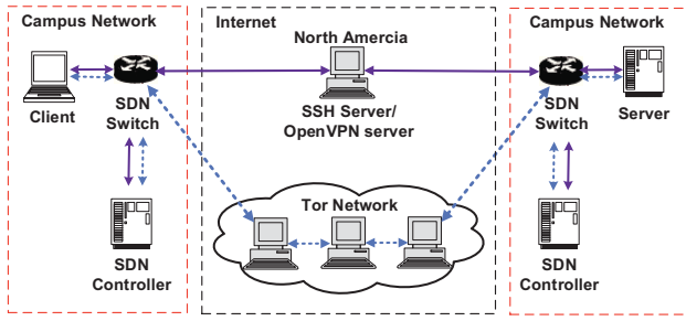
Fig. 3. Experiment setup
