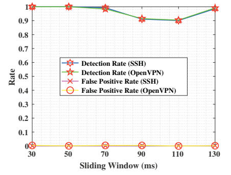
Fig. 6. Detection rate for SSH and OpenVPN versus Sliding Window
