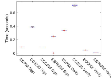
Fig. 6: ECC signature operations
