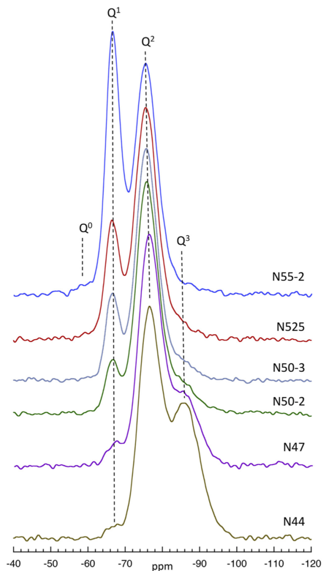
Fig. 1. ^{29}\text{Si} MAS NMR spectra of sodium silicate glasses with natural isotopic abundance. Sample numbers are based on nominal compositions: analyzed compositions are slightly different (see Table 1). Here and in Figs. 2 and 3, intensities are normalized to that of the central \text{Q}^2 peak.
