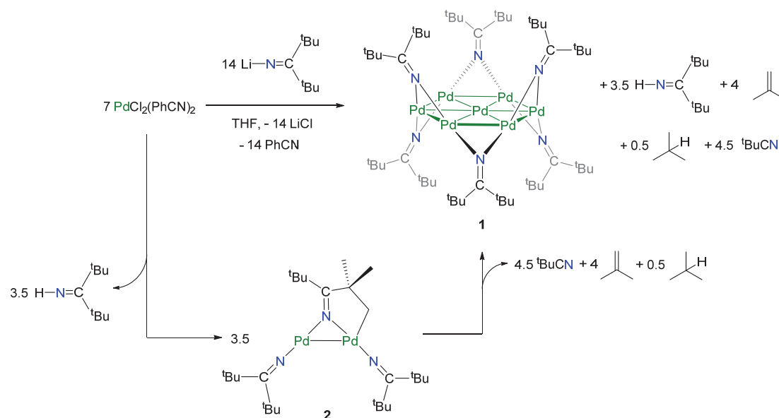
Scheme 1. Synthesis of the palladium nanosheet \text{Pd}_7(\text{N}=\text{C}^t\text{Bu}_2)_6 ( 1 )
