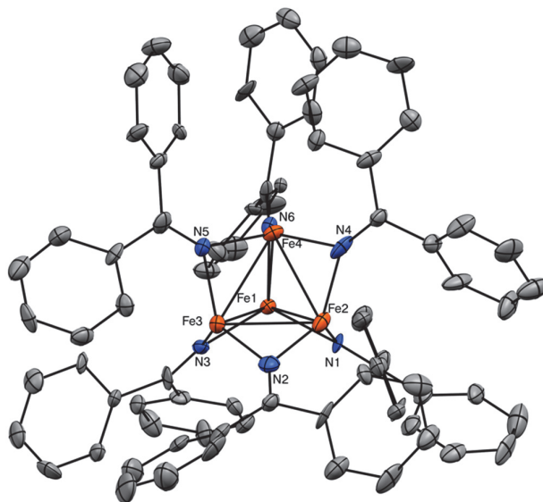
Figure 1. ORTEP diagram of one independent molecule of 1 with 50% probability ellipsoids. Hydrogen atoms, toluene solvates, and a second molecule of 1 are omitted for clarity. Color legend: Fe = orange; N = blue; C = grey.
