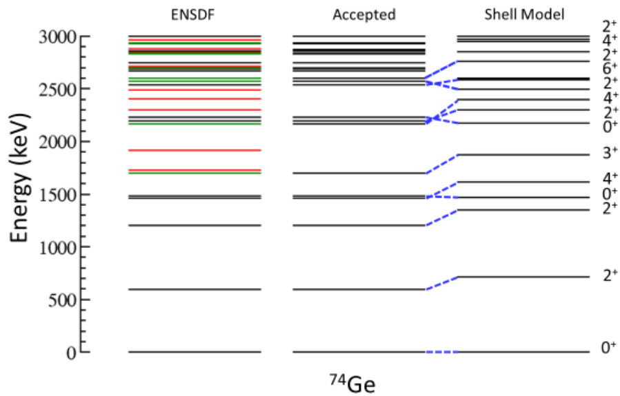
Figure 4. Comparison of accepted (center) low-lying levels in ^{74}\text{Ge} with the ENSDF compilation (left) [16] and a shell model calculation (right) [15]. See caption of figure 1 for color-coding details.
