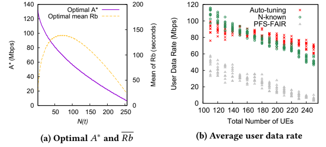
Figure 16: Simulation results with \phi_n/DDL_n = 0.25 . (a) The throughput threshold decreases as the number of CASTLE users increases. (b) CASTLE Auto-tuning outperforms PFS-FAIR, while it is comparable to CASTLE N-known.
