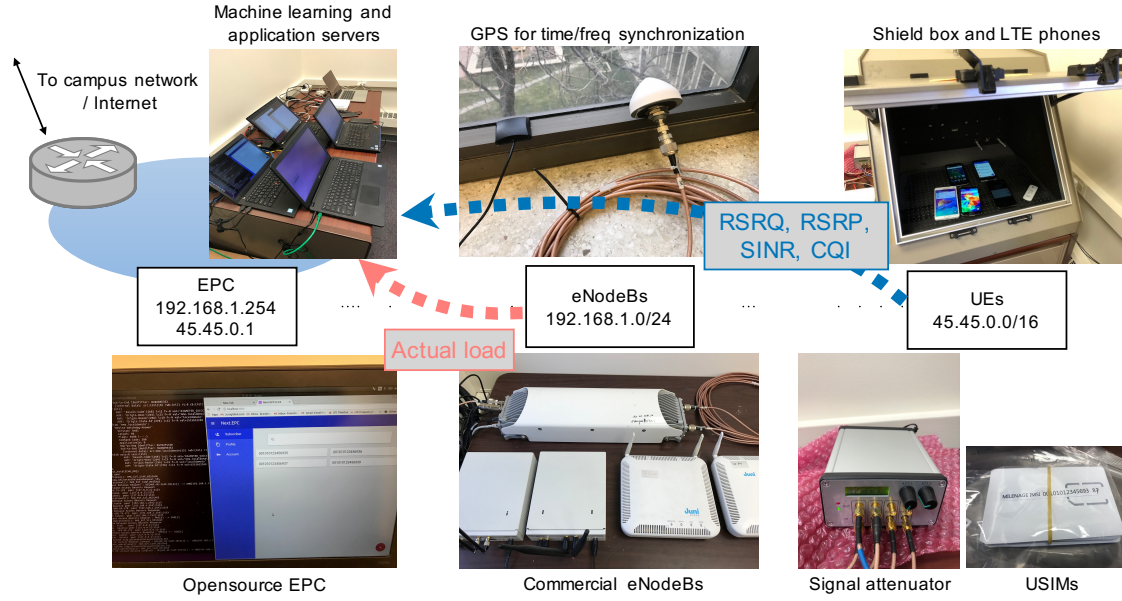
Figure 5: Our controllable end-to-end LTE network testbed composed of eNodeBs, UEs, an EPC, a signal attenuator, and a shield box. We used 2x LTE Band3 FDD eNodeBs and 10x LTE phones for the experiments.
