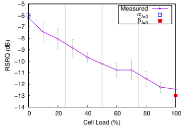
Figure 6: Measured average RSRQ in idle channel as a function of cell load.
