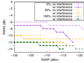
Figure 7: Measured RSRQ with co-channel interference.
