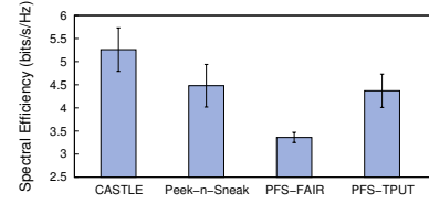
Figure 13: CASTLE shows better spectral efficiency when the UEs are stationary by 17%, 57%, and 20%, compared to Peek-n-Sneak, PFS-FAIR, and PFS-TPUT, respectively.
