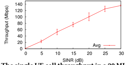
Figure 3: The single UE cell throughput in a 20 MHz channel. Measured with a Motorola G5 Plus, Samsung Galaxy S5, and Samsung Galaxy Note4.
