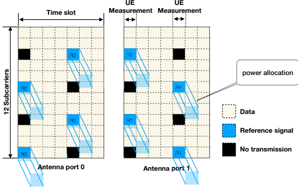
Figure 4: One RB consists of 12 subcarriers ( 12 \times 15 KHz) in the frequency domain and one slot (0.5 ms) in the time domain. Power is allocated only to 2 REs of the reference signal per antenna in a UE measurement.
