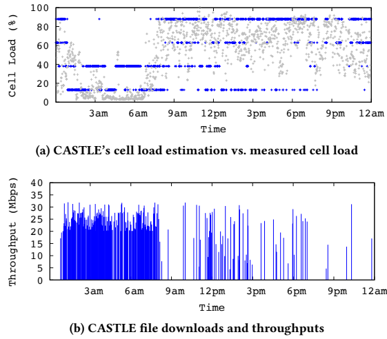
Figure 17: Tested at the edge of a real AT&T cell operating on 739 MHz where the average RSRP was -110 dBm. (a) A blue dot depicts one of four cell load classes estimated by CASTLE, while gray dots are the measured loads. (b) A single vertical line depicts a file transfer done by CASTLE. Our CASTLE application effectively leverages the time when there was not much load in the early morning.
