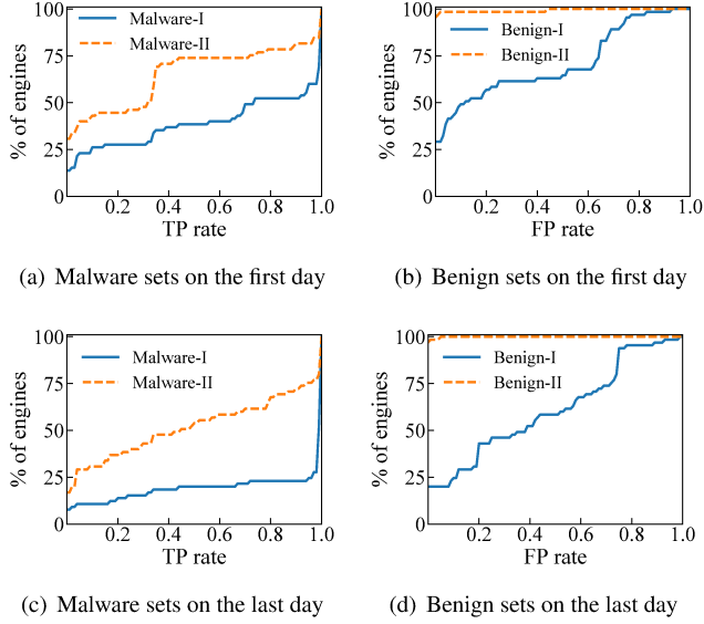
Figure 12: CDF plots of the true positive (TP) rate and the false positive (FP) rate of each engine.
