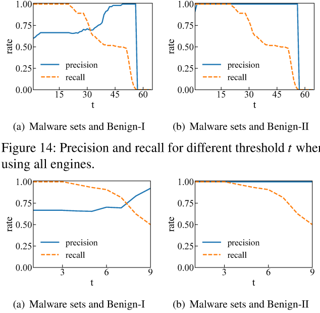
Figure 15: Precision and recall for different threshold t when only using reputable engines.
