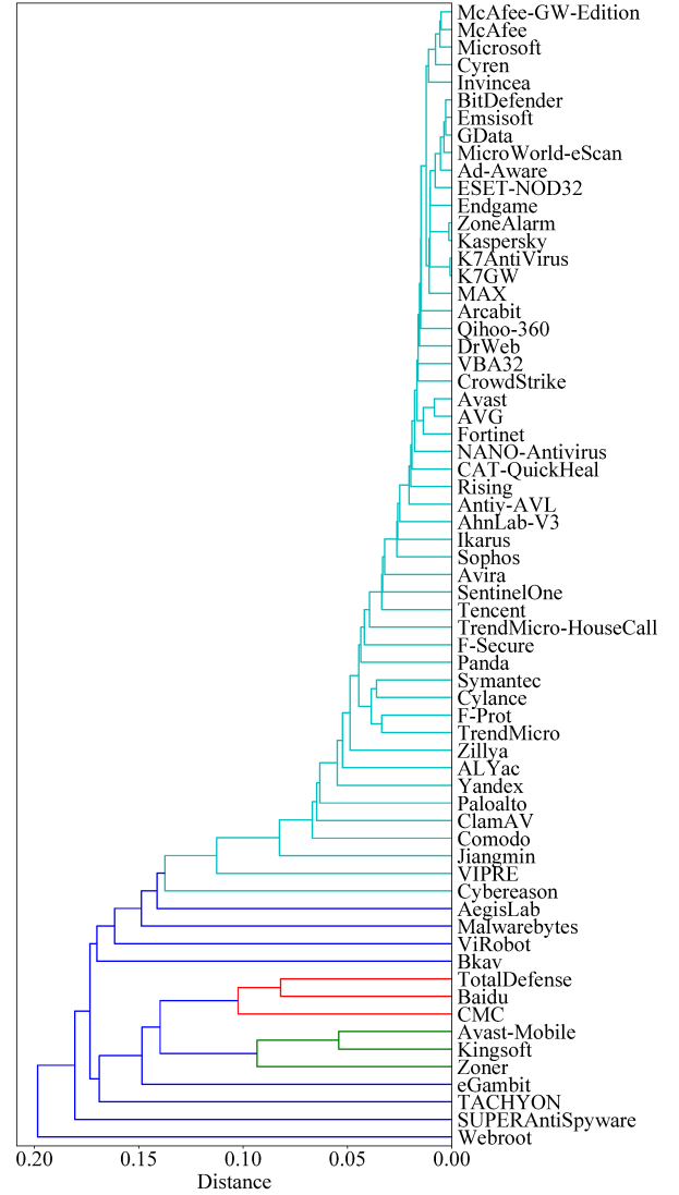
Figure 18: The dendrogram of engine clusters. x -axis shows the distance threshold. A shorter distance indicates two engines have more similar label sequences. Clusters with distance shorter than the threshold are gradually merged together.
