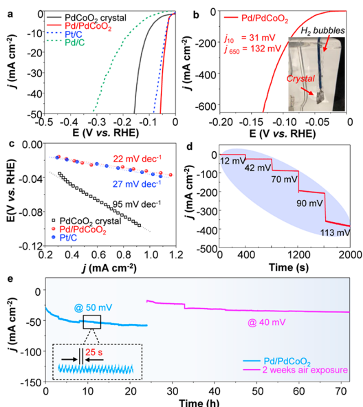
Figure 2. (a) Polarization curves of the modified bulk \text{PdCoO}_2 single crystal and 20% Pt/C, Pd/C commercial catalysts. (b) Polarization curves of the bulk \text{PdCoO}_2 single crystal at larger applied overpotential. The inset shows the produced hydrogen bubbles on the crystal surface. (c) Tafel plots of the bulk \text{PdCoO}_2 single crystal catalysts and 20% Pt/C catalyst. (d) Multicurrent process showing the current density increasing from 5 to 350 \text{ mA cm}^{-2} without iR correction. (e) Current versus time over 24 h showing a constant potential of -50 \text{ mV} , which is reduced to -40 \text{ mV} (for 48 h) after 2 weeks of exposure to air.
