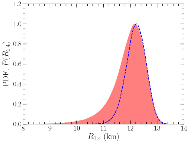
Fig. 12. Probability distribution (red) for the radius of a 1.4 M_\odot neutron star from the Bayesian analysis in the present work. The blue dashed line represents the probability distribution when we include in our posterior for R_{1.4} the M = 2.17^{+0.11}_{-0.10} M_\odot observation [63].
