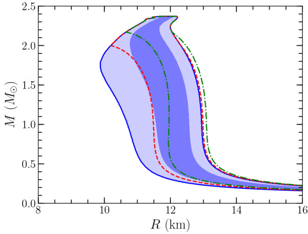
Fig. 7. The blue band shows the 95% (68%) credibility range for the mass-radius relationship of neutron stars obtained within the present Bayesian modeling of the nuclear equation of state. The red dashed curve area is obtained when we include only those equations of state that produce mass of neutron stars greater 2.0 M_{\odot} neutron stars. The green dot-dashed curve indicated 95% credibility when we include the EOS which can make 2.17 M_{\odot} neutron stars.
