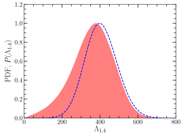
Fig. 14. Probability distribution (red) for the tidal deformability of a 1.4 M_\odot neutron star obtained from the 300000 equations of state generated from the posterior distribution in our Bayesian modeling. The blue dashed line represents the probability distribution when we include in our posterior for \Lambda_{1.4} the M = 2.17^{+0.11}_{-0.10} M_\odot observation [63].
