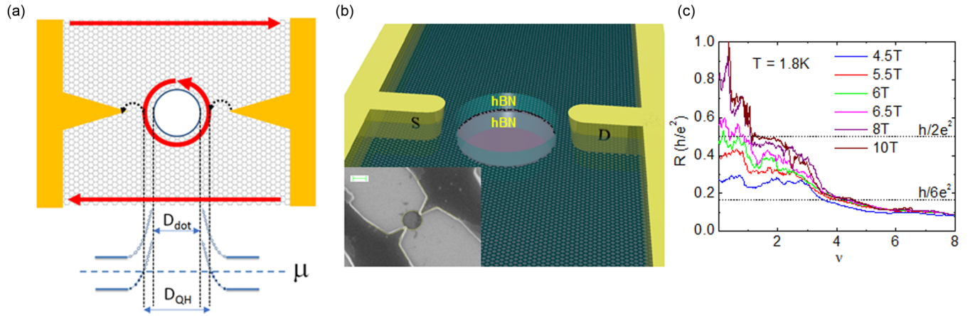
FIG. 1. Graphene QH antidot. (a) Schematics of QH antidot. The red arrows indicate the QH edge states. The band structure illustrates the bulk LLs and the quantized edge states. (b) Structure of a point-contact coupled QH antidot on graphene/hBN heterostructure. Inset: SEM image of a 310-nm-diameter antidot sample. The yellow dotted lines highlight the boundaries of the antidot and the side contacts. The scale bar is 200 nm. The bulk channel edges are outside the view. (c) Two-terminal resistance as a function of filling factor, measured in various fixed magnetic fields by ramping the back-gate voltage.
