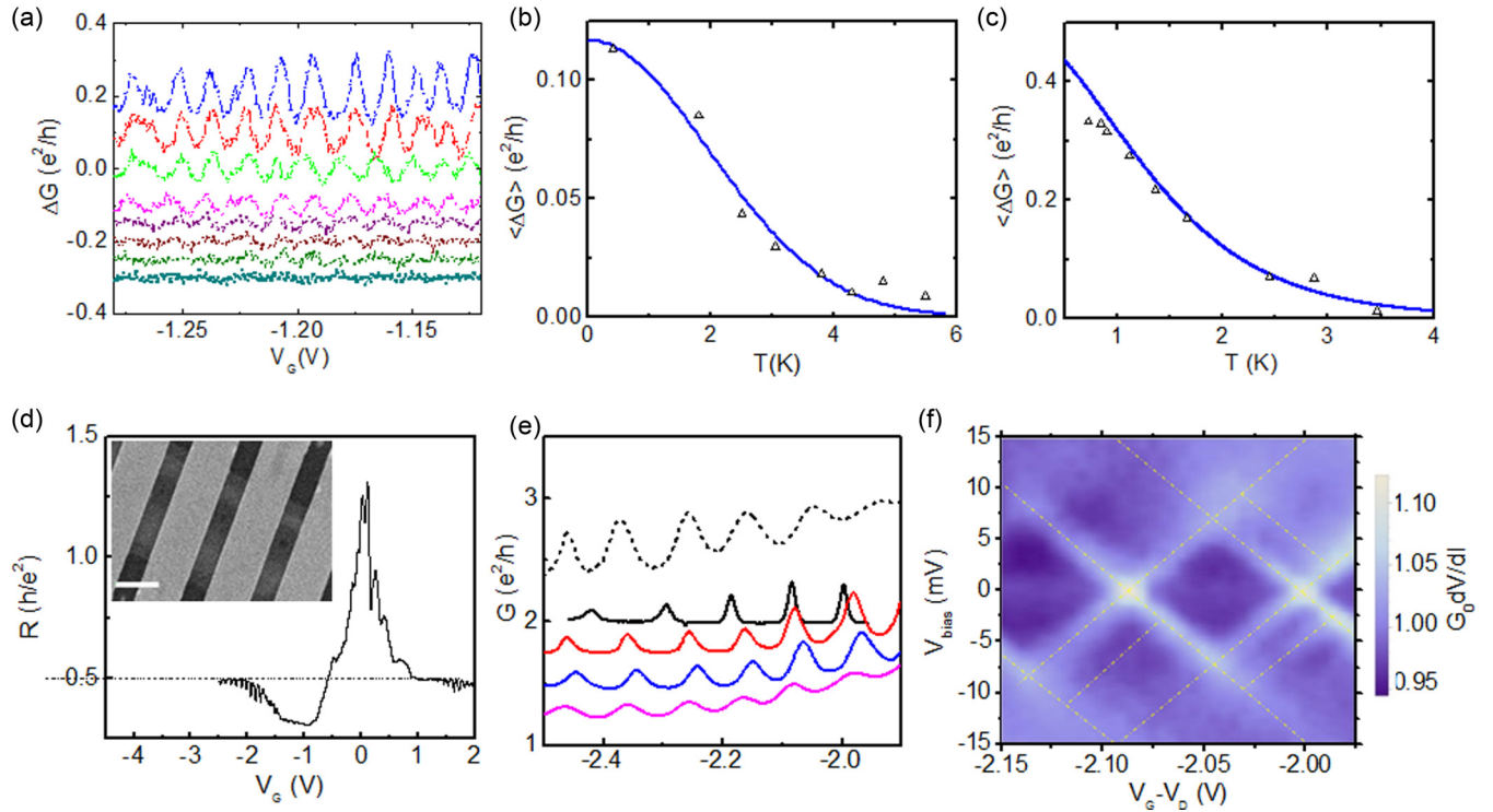
FIG. 4. Thermal suppression of conductance oscillations in the QH antidots. (a) Gate-dependent conductance oscillation at various temperatures. The curves, taken at (from top to bottom) T = 0.4, 1.8, 2.5, 3.1, 3.8, 4.3, 4.8 , and 5.5 K, are vertically shifted for clarity. The temperature dependence of the averaged conductance oscillation amplitude for the weakly coupled 310-nm antidot (b) and the strongly coupled 200-nm antidot (c) are fitted with thermal excitation models. (d) Conductance oscillations in a suspended graphene QH antidot at B = 1 T. The dotted line labels QH plateau resistance at n = 2 . Inset: SEM image of a suspended graphene with three QH antidot devices. The scale bar is 1 \mu\text{m} . (e) Temperature dependence of conductance oscillations. The dotted and the solid black curves, both measured at 450 mK, correspond to before and after thorough current annealing, respectively. The red, blue, and purple curves are taken at 2, 5, and 10 K, respectively, and are shifted downward for clarity. (f) Charge-stability plot for the suspended graphene QH antidot, taken in 1-T magnetic field at 450 mK. The dotted lines are guides to the eyes.
