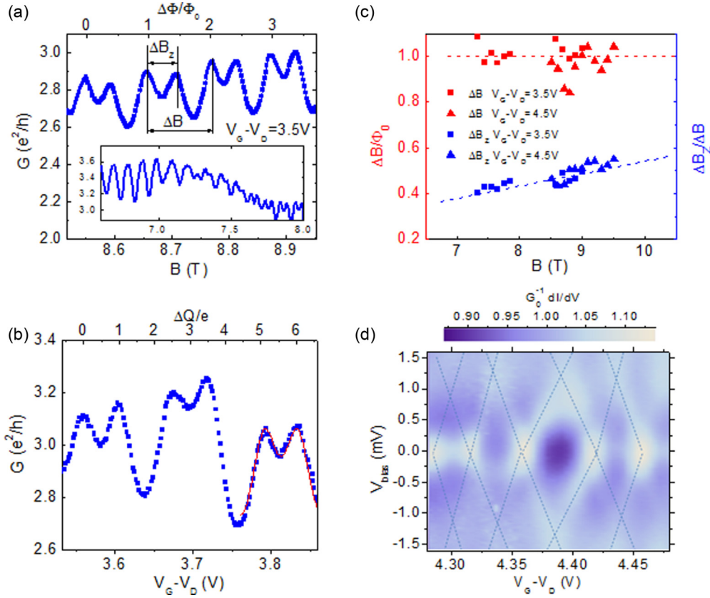
FIG. 3. AB oscillations in strongly coupled QH antidot. (a) Conductance oscillations showing \Phi_0 flux period and Zeeman splitting. Inset: In lower magnetic fields, the conductance oscillation evolves from merged peaks with \Phi_0 period to M-shaped spin-resolved oscillations, with increasing magnetic field. (b) Conductance oscillations with ramping gate voltage. The top x axis shows the change in charge number calculated using the geometrical capacitance over the physical area of the antidot. The red solid curve shows the fitting to a relatively symmetric M-shaped oscillation using thermal excitation model. (c) Magnetic-field dependences of the AB oscillation period ( \Delta B ) and normalized Zeeman splitting ( \Delta B_z/\Delta B ). The dotted lines are guides to the eyes. (d) Differential conductance versus bias voltage and gate voltage. Dotted lines are guides to the eyes. From the bias- and gate dependence of the differential conductance, the energy-level spacing is a summation of the bias voltages at the two adjacent diamond tips which correspond to the two spin states.
