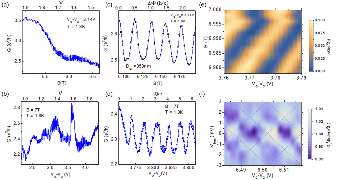
FIG. 2. Coulomb blockade in relatively weakly coupled QH antidot. Conductance oscillations are observed with ramping magnetic field (a) and gate voltage (b). (c) A zoom-in of the conductance oscillations shows a magnetic flux period of \Phi_0/2 , calculated using a QH edge-state diameter of D_{\text{QH}} = 350 nm. (d) A zoom-in of the conductance oscillations shows approximate one oscillation per charge, with charge number calculated using the geometric capacitance over the physical area of the antidot. (e) Conductance oscillations versus both gate voltage and magnetic field. (f) Charge-stability diagram showing Coulomb-blockade characteristics. The dotted lines are guides to the eyes.
