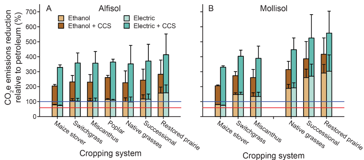
Figure S3. CO 2 e emission reduction for alternative cellulosic biofuel cropping systems used for ethanol or electricity with and without carbon capture and storage (CCS) to power vehicles, before SOC equilibration to higher levels. The red horizontal line represents the 60% reduction currently required for U.S. designation as an advanced biofuel. The blue horizontal line represents the 100% reduction threshold for negative CO 2 e emissions. Values are means \pm standard errors (n=4 Alfisol or 5 Mollisol replicate blocks).
