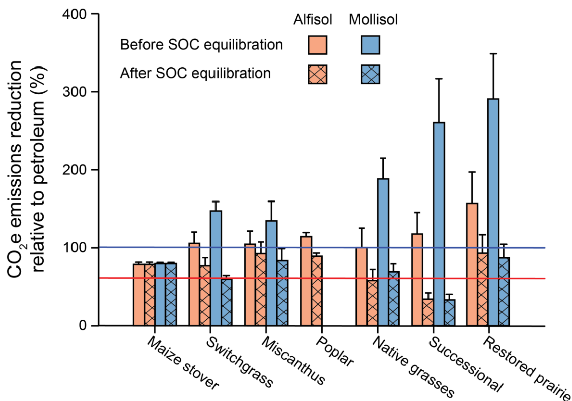
Figure S2. Anticipated CO 2 e emission reduction relative to petroleum before and after long-term SOC equilibration to higher levels, assuming ethanol production to power vehicles (scenario 1 – see Materials and Methods). The left-hand bar of each Mollisol and Alfisol pair is the same as in Fig. 3a. The cross-hatched right hand bar in each pair represents CO 2 e emission reduction after long-term SOC equilibration, which is likely to take 30-50 years assuming no change in primary productivity (energy production potential). The red horizontal line represents the 60% reduction currently required for U.S. designation as an advanced biofuel. The blue horizontal line represents the 100% reduction threshold for negative CO 2 e emissions. Values are means \pm standard errors (n=4 Alfisol or 5 Mollisol replicate blocks).
