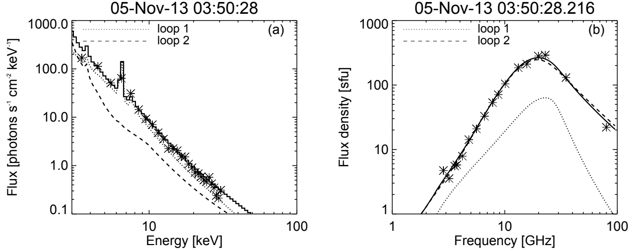
Figure 8. (a) The observed RHESSI X-ray spectrum for time interval 03:50:28-03:50:32 UT (asterisks) and the corresponding simulated spectrum (histogram) from the 3D model; (b) the same for the radio domain with NoRP and SRS data at 03:50:28 UT (asterisks) and the simulated microwave spectrum (black solid line). The dotted and dashed lines correspond to contribution from loop 1 and loop 2 separately to the X-ray and the radio simulated spectra.
