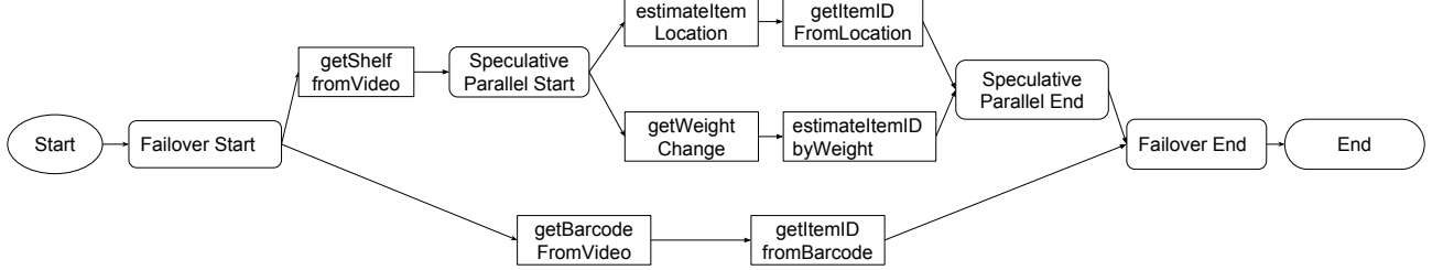
Fig. 9. Generated Workflow for Use Case 1
