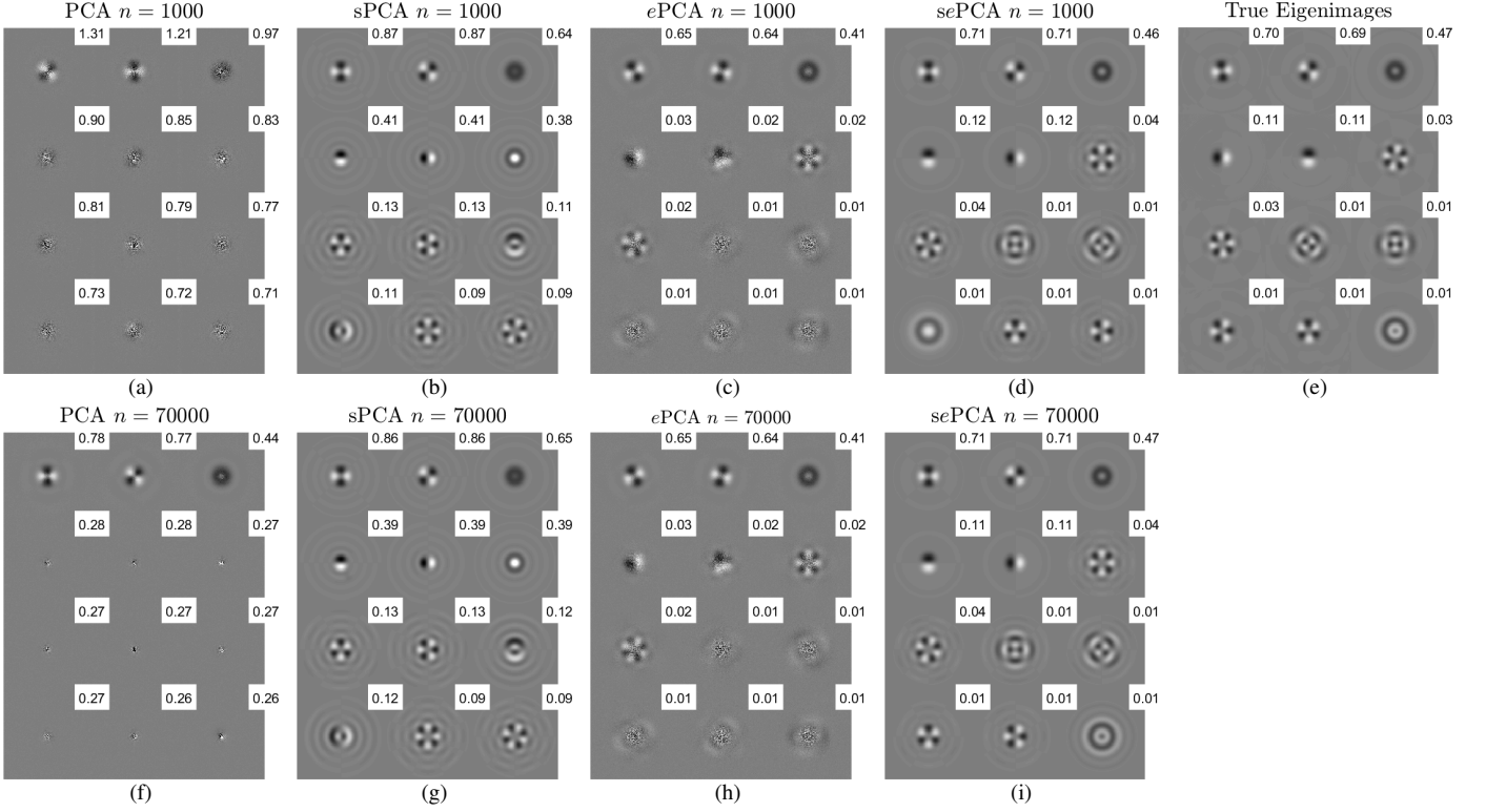
Fig. 3: Eigenimages estimated from noisy XFEL data using PCA, steerable PCA (sPCA), ePCA, and steerable ePCA (sePCA), ordered by eigenvalues. Input images are corrupted by Poisson noise with mean photon count 0.01 (shown in Figure 1b).
