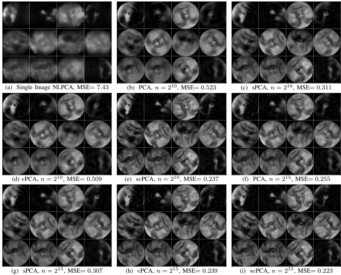
Fig. 11: Sample denoised images from Yale Face Database B illustrated in Fig. 7 using NLPKA, PCA, sPCA, ePCA, and sePCA. Image size is 64 \times 64 . The intensity range is [0, 2.6] for (a), and is [0, 11.1] for (b)–(i).
