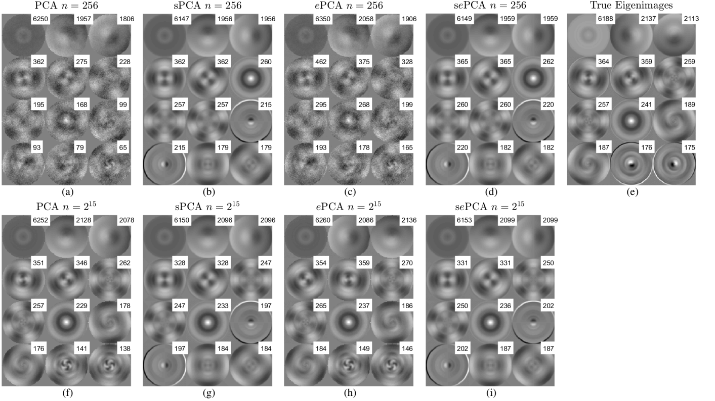
Fig. 8: Eigenimages estimated from noisy rotated Yale Face Database B using PCA, sPCA, ePCA, and sePCA, ordered by eigenvalues. Input images are corrupted by Poisson noise with mean intensity 2.3 photons per pixel (shown in Fig. 7b).
