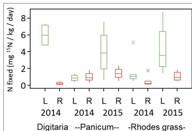
FIGURE 1 | Nitrogen fixation potential for the leaf (L) and root (R) samples of different perennial grasses estimated using a laboratory ^{15}\text{N} -incubation assay. Based on minimum \delta^{15}\text{N} (‰) value for detection of \text{N}_2 fixation, the minimum detectable N fixation rate was 0.10 \text{ mg N fixed kg}^{-1} \text{ day}^{-1} .
