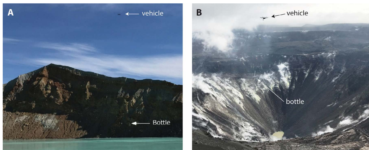
Figure 18: Water sampling, [A] at Yugama crater lake (reproduced from [Terada et al. 2018] under the Creative Commons Attribution 4.0 International License) and [B] at Halema'uma'u, Kilauea, 2019.
