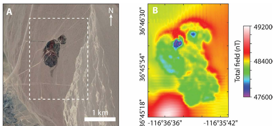
Figure 7: UAS magnetic survey data collected using a DJI Matrice 100 with dual triaxial fluxgate sensors (SENSYS MagDrone R3; Figure 1G). [A] Overview imagery (© 2020 Maxar Technologies, Google Earth) of the survey area (dashed box) of Little Cones, Amargosa Valley, Nevada, USA, illustrating the limited surface exposure of black volcanic rocks. [B] Interpolated magnetic map of preliminary field data prior to correction for UAS vehicle heading. Buried lava is revealed by the irregularly shaped central area of low total magnetic field (mainly green and blues) which result from the reverse polarisation of the volcanic rocks.
