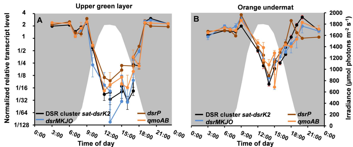
FIGURE 8 | Relative transcript levels (y-axis) of DSR-affiliated genes grouped according to the MS contig gene composition shown in Figure 5 across a diel cycle (x-axis) in (A) MS upper green layer, and (B) MS undermat. Black lines represent relative transcript levels of genes sat-aprAB-qmoC-dsrABCDKLMN ; blue lines represent genes dsrMKJO ; brown lines represent dsrP ; orange lines represent qmoAB . White areas indicate light periods during the day and irradiance intensities in \mu\text{mol photons m}^{-2} \text{s}^{-1} (400–700 nm, secondary y-axis), while gray areas indicate dark periods during the night.
