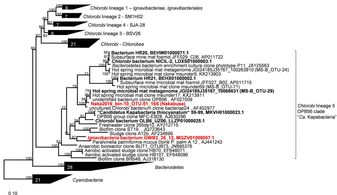
FIGURE 4 | Maximum-likelihood tree of 16S rRNA gene sequences derived from the metagenome bins analyzed in this study and closely related partial genomes showing their phylogenetic affiliation with the "Chlorobi lineage 5" (OPB56 clade, "Ca. Kapabacteria"). Percentage numbers on nodes refer to 100 bootstrap pseudo-replicates conducted. Only values >50% are shown. Scale bar represents 0.1 changes per nucleotide position.
