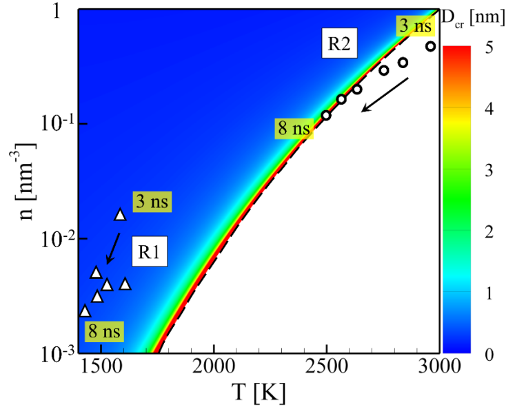
Figure 10. The contour plot outlining the critical (minimum) diameter of particles that can grow by condensation from the surrounding vapor under specific temperature and Ag vapor density conditions calculated based on the Gibbs-Kelvin equation. The dashed line shows the saturation condition for flat vapor-liquid interface. The blue part of the field corresponds to conditions when all nanoparticles can grow by condensation, while the white area corresponds to conditions where particles of any size should evaporate. The conditions realized in sub-regions R1 and R2, summarized in Table 1, are shown as triangles ( n_{R1}, T_{R1}^{1nm} ) and circles ( n_{R2}, T_{R2}^{1nm} ).
