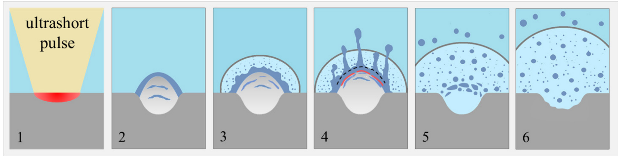
Figure 1. Schematic illustration of the sequence of dynamic processes triggered by irradiation of a metal target by an ultrashort (femtosecond to tens of picosecond) laser pulse . The liquid water is colored blue, the metal target is grey, the ablation plume is light grey, and the expanding cavitation bubble is light blue. The metal nanoparticles and a transient molten metal layer generated at the plume-water interface are shown in dark blue color. The metal nanoparticles and a transient molten metal layer generated at the plume-water interface are shown in dark blue color. The red curves in panel 4 show schematically the backside impacts from large (spalled) metal droplets joining the hot molten metal layer formed at the ablation plume-water interface. The impacts generate pressure pulses (shown by dashed curves) that induce jetting of the molten metal (Richtmyer-Meshkov instability) from the layer roughened by Rayleigh-Taylor instability of the plume-water interface. The schematic is informed by large-scale atomistic simulations reported in Refs. 8, 40, and 41.
