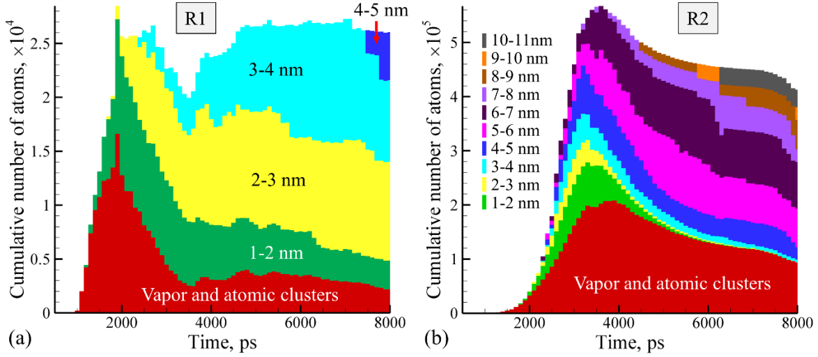
Figure 8. Results of the analysis of nanoparticles generated in a simulation illustrated by Figures 3-7: The cumulative numbers of atoms that belong to the vapor phase and atomic clusters with diameters less than 1 nm (red color), and nanoparticles of different sizes (color coding defined in the legend) identified at different times during the simulation in sub-regions (a) R1 and (b) R2 defined in Figure 3. Large nanoparticles produced as a result of decomposition of a transient interfacial layer illustrated in Figure 6 are not included in the analysis illustrated by this figure.
