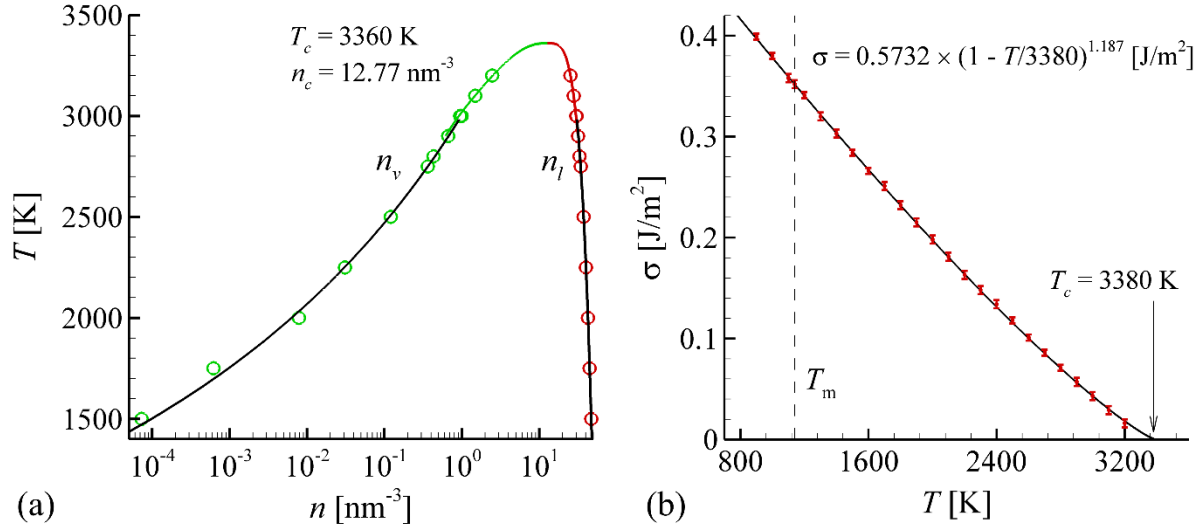
Figure 13. The temperature – density ( T - n ) plane of the liquid-vapor part of the phase diagram (a) and the temperature dependence of surface tension (b) calculated for the model EAM Ag used in the simulations of PLAL reported in this paper. In (a), the black curves are the parts of the binodal curves obtained by direct fitting to the results of liquid-vapor coexistence simulations shown by green and red points; the red and green curves represent the fitting of the data points to the dependences predicted from renormalization group theory for the material behavior near the critical point. 74,75 The critical density n_c = 12.77 \text{ nm}^{-3} obtained from the fitting, corresponds to \rho_c = 2.29 \text{ g/cm}^3 . In (b) the error bar corresponds to the standard error.
