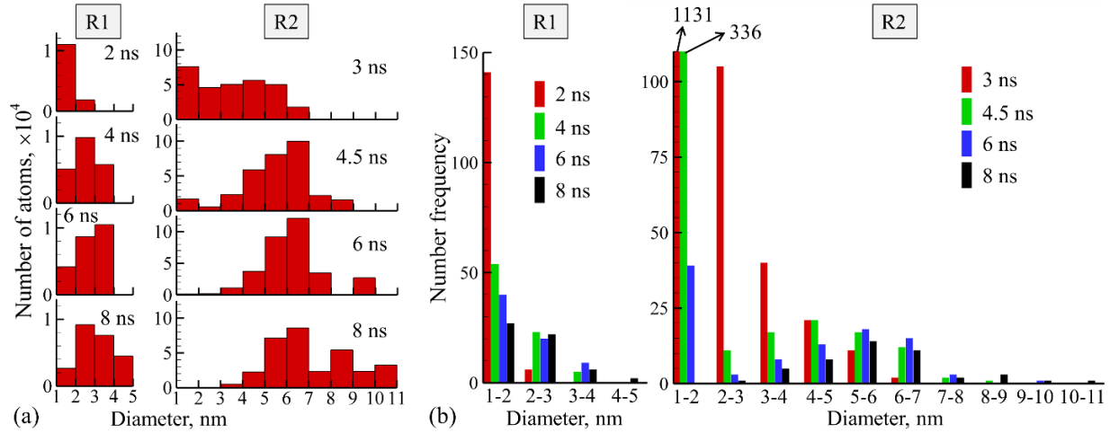
Figure 9. Results of the analysis of nanoparticles generated in a simulation illustrated by Figures 3-7: Nanoparticle size distributions shown for different times during the simulation in the form of (a) the number of atoms in nanoparticles of different sizes (above 1 nm) and (b) number frequency of the nanoparticles. The distributions are calculated separately for sub-regions R1 and R2 defined in Figure 3. Large nanoparticles produced as a result of decomposition of a transient interfacial layer illustrated in Figure 6 are not included in the distributions.
