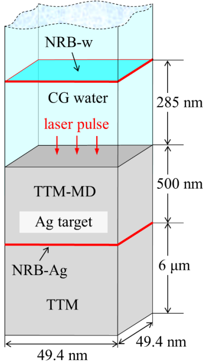
Figure 2. Schematic representation of the initial system used in simulations of short pulse laser interaction with a bulk Ag target in water. The top part of the Ag target (shown by grey color) is represented by TTM-MD model, whereas the temperature evolution in the deeper part of the target is described by TTM equations. A 285-nm-thick layer of water adjacent to the metal target is represented by a coarse-grained MD model (CG water). At the bottom of the TTM-MD domain and on the top of the CG water region, the non-reflecting propagation of the laser-induced pressure waves is reproduced by acoustic impedance matching boundary conditions denoted as NRB-Ag and NRB-w, respectively. In the lateral directions, parallel to the irradiated surface, periodic boundary conditions are applied. The dimensions of the computational system marked on the schematic are used in the simulation of 400 ps pulse laser irradiation discussed in Section 3.1. A smaller system with lateral dimensions of 4.94 \text{ nm} \times 4.94 \text{ nm} is used in the simulations performed for longer pulse durations of 1 and 2 ns and reported in Section 3.2.
