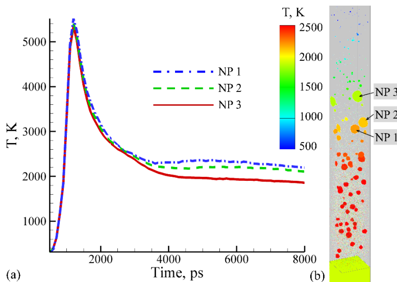
Figure 7. The time dependence of the temperatures of groups of atoms that end up in the three large nanoparticles produced through the disintegration of the transient dense layer formed at the plume-liquid interface (a), and a snapshot of the final configuration taken at a time of 8 ns, with atoms colored by local temperature (b).
