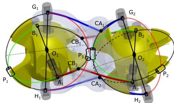
Fig. 9 The segment design capturing the mechanism in Fig. 6(b)
