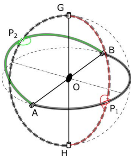
Fig. 5 The illustration of the two sets of the cable case. The lines from G to H through P_1 belong to one solid body. The lines from A to B through P_2 belong to another solid body. The transparent thick solid lines belong to one cable routing profile. The transparent thick dashed lines belong to the other cable routing profile.
