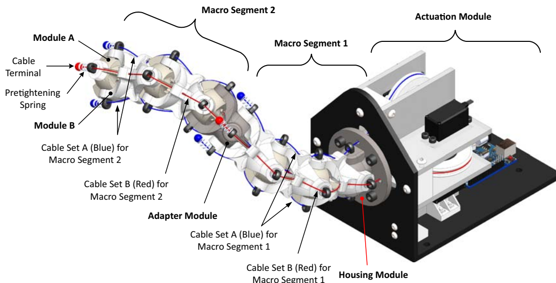
Fig. 7 Complete assembly of the RML tail without the extensional springs
