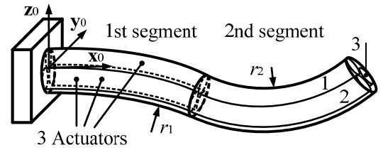
Figure 1: Illustration of a two-segment constant curvature continuum robot with three intrinsic actuators in each segment
