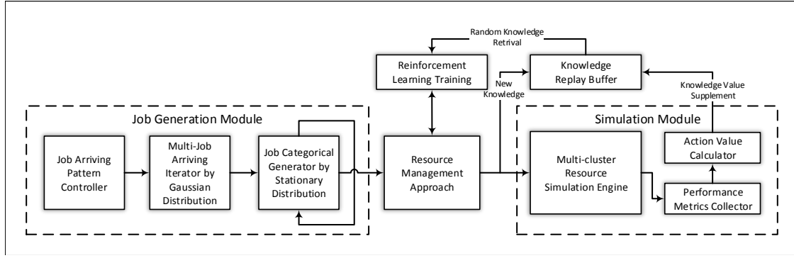
Figure 2. Reinforcement learning procedure in single episode.
