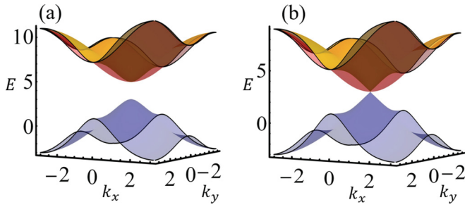
FIG. 7. (a) Similar to Fig. 1(a) but plotted with symmetry breaking terms such that t_x = 1 , t_y = 0.5 , t_{\text{SO},x} = 1 , and t_{\text{SO},y} = 0.5 . (b) With such an anisotropy, the 2D triply degenerate point now occurs at \delta_T = 6 .
