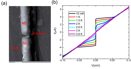
FIG. 1: (Color online) (a) Scanning electron microscopy SEM image of one of the studied devices, junction-1, made with two Nb leads \sim 100 nm apart on a polished crystal of SmB 6 . (b) Current-voltage I-V characteristics of the junction-1 for a set of temperatures. The supercurrent persists up to 3.6 K.
