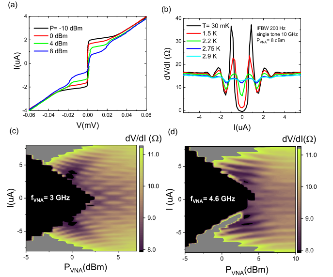
FIG. 2: (Color online) (a) AC Josephson effect giving rise to Shaphiro steps in IV and (b) corresponding peaks in differential resistance for another sample, junction-1. (c) and (d) Color plots demonstrating such steps for junction-2 at two different frequencies.
