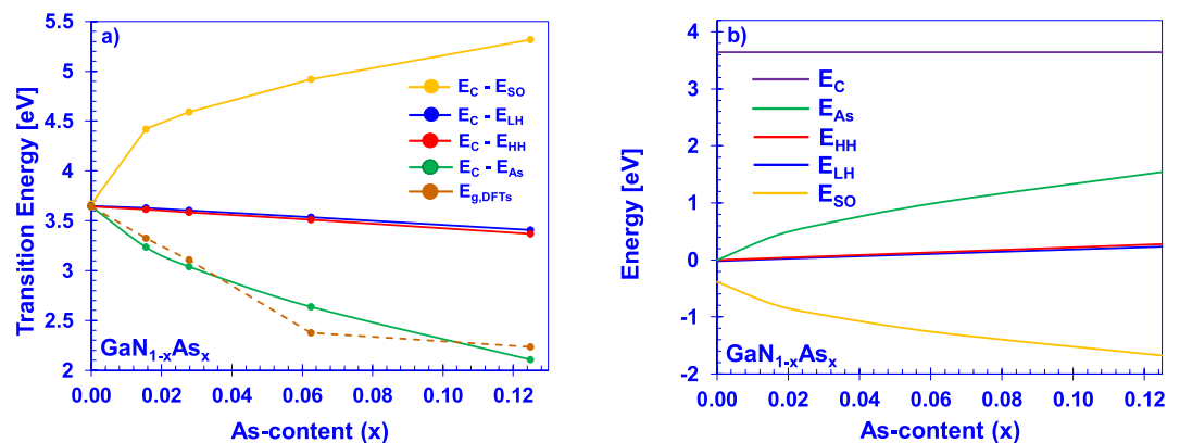
Figure 3. Best-fit valence (a) subband transition energies and DFT-calculated reduction of band gap and, (b) subband positions, at the gamma point via the BAC model using parameters E_{As} = -0.39 eV and C_{GaNAs} = 2.57 eV.
