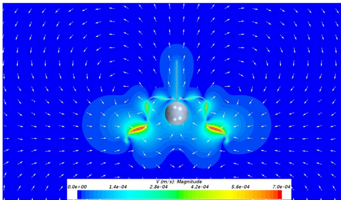
Figure 14. Snapshot of flow field generated by swimming haptophyte, Pymnesium polylepis , computed by CFD. The simulation is based on the observed kinematics and beat pattern of the two flagella. The straight, slender structure in front of the cell is the haptone (not a flagellum) that is involved in prey capture. Simulation by Seyed Saeed Asadzadeh (DTU).
