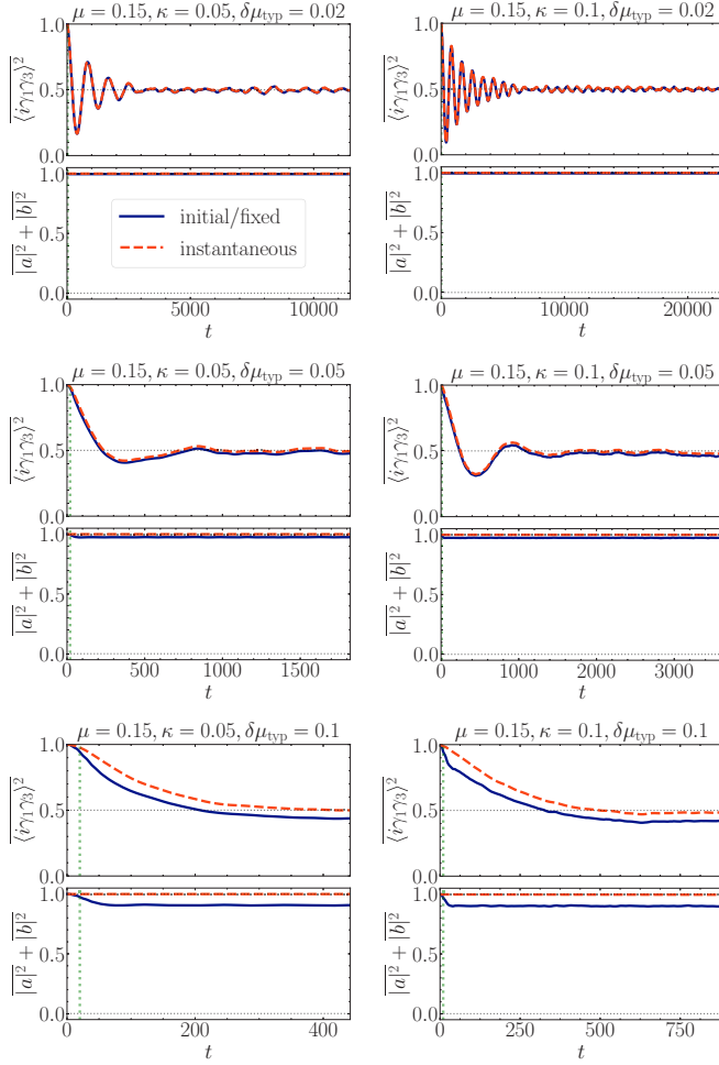
FIG. 10. Measurements of \langle \gamma_1 \gamma_3 \rangle^2 and |a|^2 + |b|^2 in both the fixed/initial (solid blue) and instantaneous (dashed orange) basis for a Kitaev tetron at \mu = 0.15 , \kappa = 0.05, 0.1 (increasing left to right), and \delta\mu_{\text{typ}} = 0.02, 0.05, 0.1 (increasing top to bottom); see text for details of other chosen parameters. Here, we initialize the system using a procedure based on the initial Hamiltonian encoded by A(t=0) . For large enough \delta\mu_{\text{typ}} , a noticeable difference in the choice of measurement basis is observed on a timescale on the order of \tau = 1/\kappa (vertical green dotted lines).
